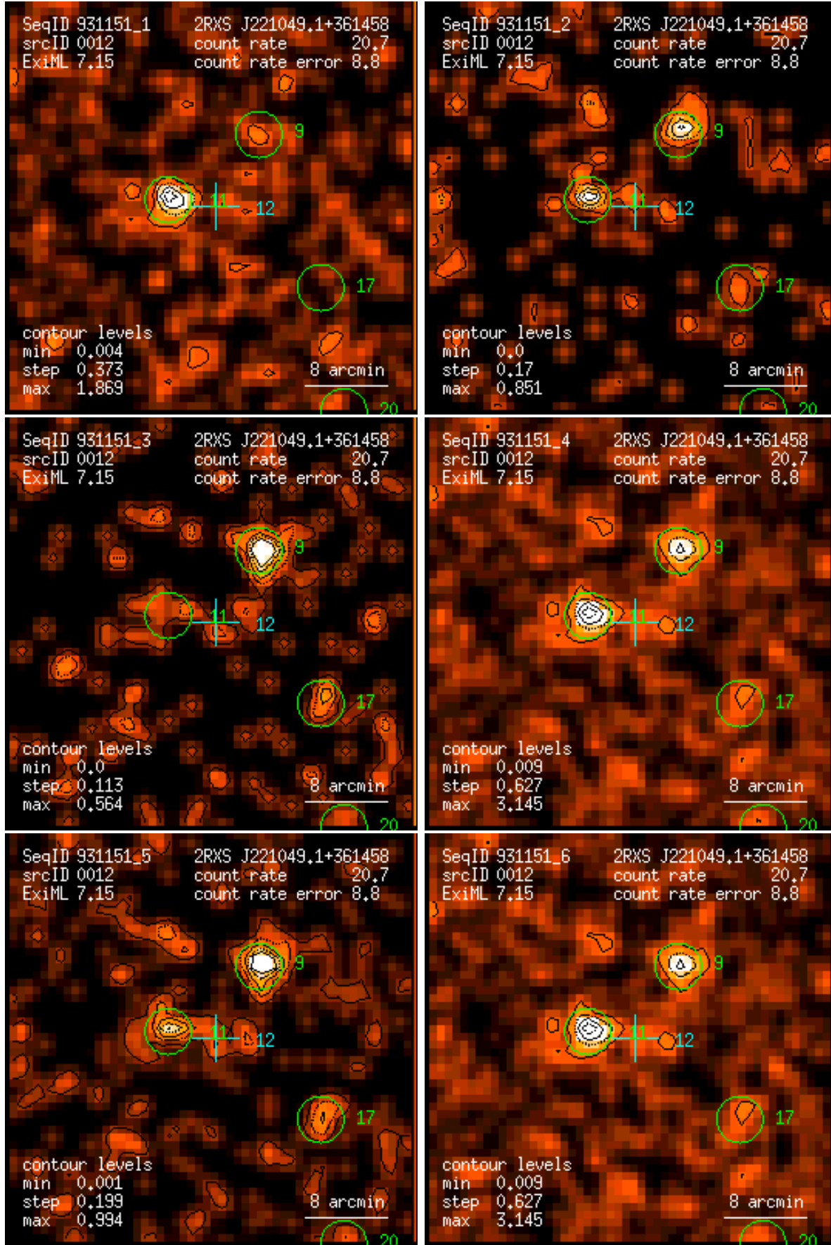
Figure 12: RASS 931151: detection 0012: band rate images, Gaussian filter: (1) PSPC channels 11 – 41, (2) 52 – 90, (3) 91 – 201, (4) 11 – 235, (5) 52 – 201, (6) 11 – 201. Broad band rates in counts/ks. Band rate contour levels in counts/ks/arcmin 2 .
