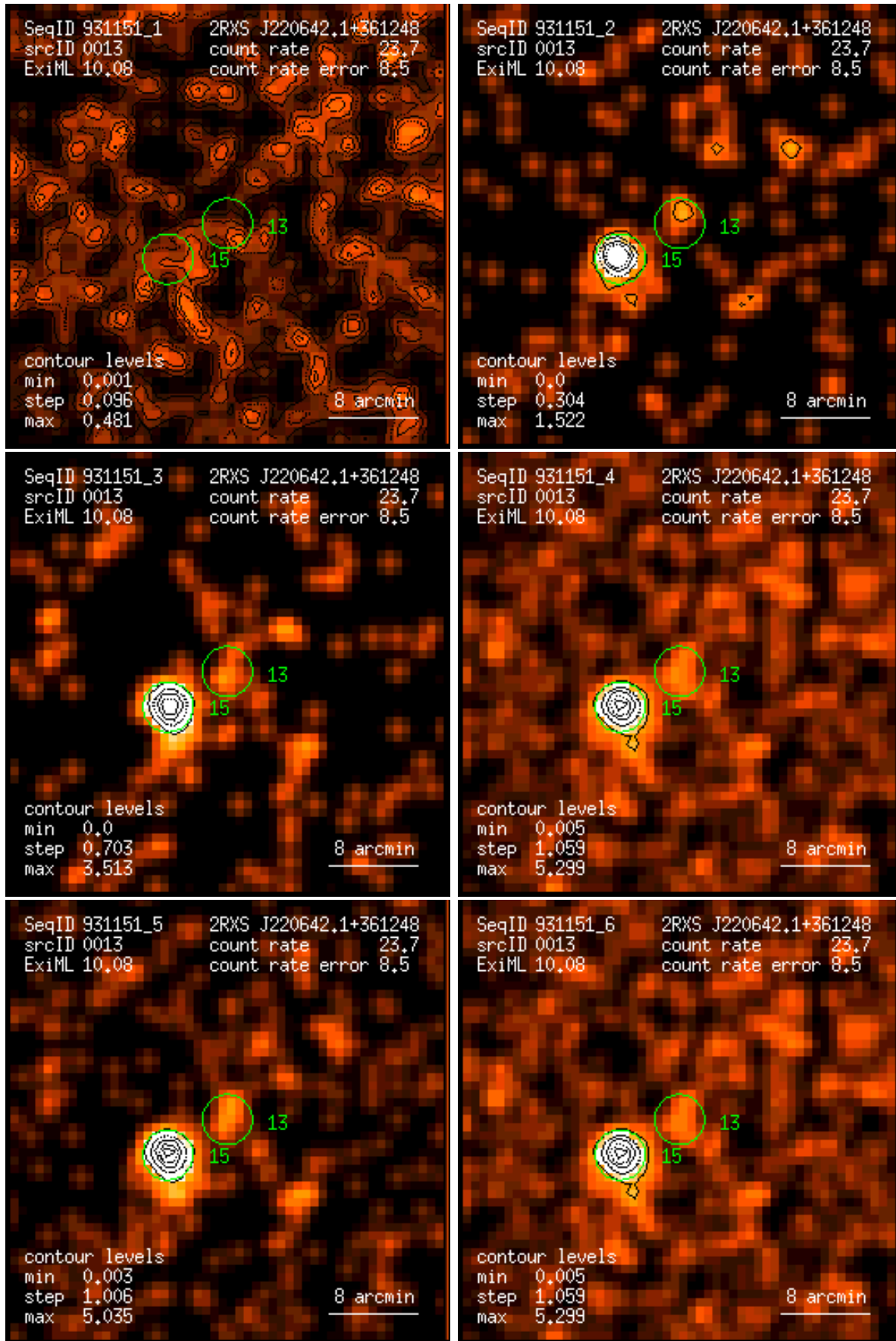
Figure 13: RASS 931151: detection 0013: band rate images, Gaussian filter: (1) PSPC channels 11 – 41, (2) 52 – 90, (3) 91 – 201, (4) 11 – 235, (5) 52 – 201, (6) 11 – 201. Broad band rates in counts/ks. Band rate contour levels in counts/ks/arcmin 2 .
