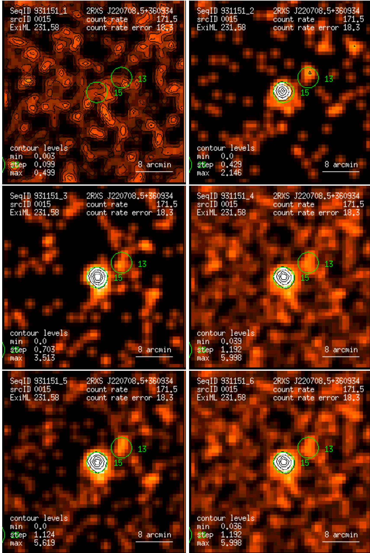
Figure 15: RASS 931151: detection 0015: band rate images, Gaussian filter: (1) PSPC channels 11 – 41, (2) 52 – 90, (3) 91 – 201, (4) 11 – 235, (5) 52 – 201, (6) 11 – 201. Broad band rates in counts/ks. Band rate contour levels in counts/ks/arcmin 2 .
