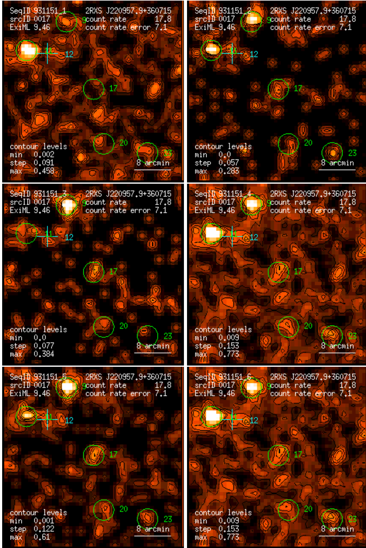
Figure 17: RASS 931151: detection 0017: band rate images, Gaussian filter: (1) PSPC channels 11 – 41, (2) 52 – 90, (3) 91 – 201, (4) 11 – 235, (5) 52 – 201, (6) 11 – 201. Broad band rates in counts/ks. Band rate contour levels in counts/ks/arcmin 2 .
