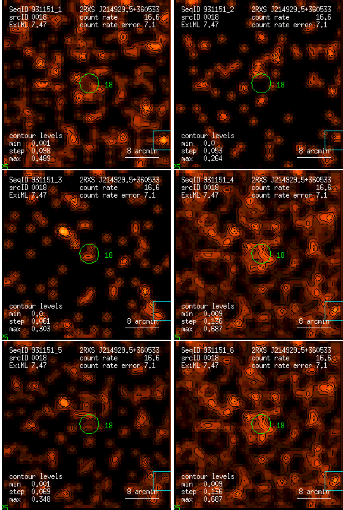
Figure 18: RASS 931151: detection 0018: band rate images, Gaussian filter: (1) PSPC channels 11 – 41, (2) 52 – 90, (3) 91 – 201, (4) 11 – 235, (5) 52 – 201, (6) 11 – 201. Broad band rates in counts/ks. Band rate contour levels in counts/ks/arcmin 2 .
