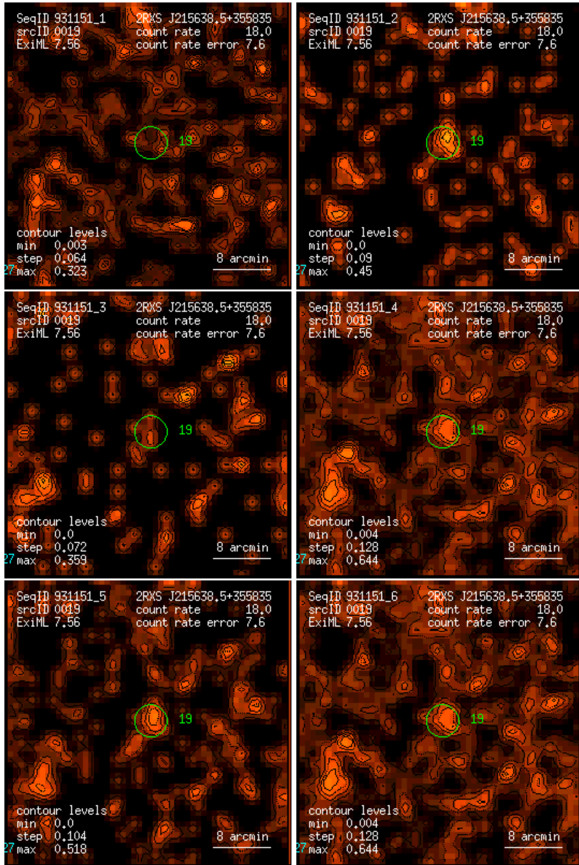
Figure 19: RASS 931151: detection 0019: band rate images, Gaussian filter: (1) PSPC channels 11 – 41, (2) 52 – 90, (3) 91 – 201, (4) 11 – 235, (5) 52 – 201, (6) 11 – 201. Broad band rates in counts/ks. Band rate contour levels in counts/ks/arcmin 2 .
