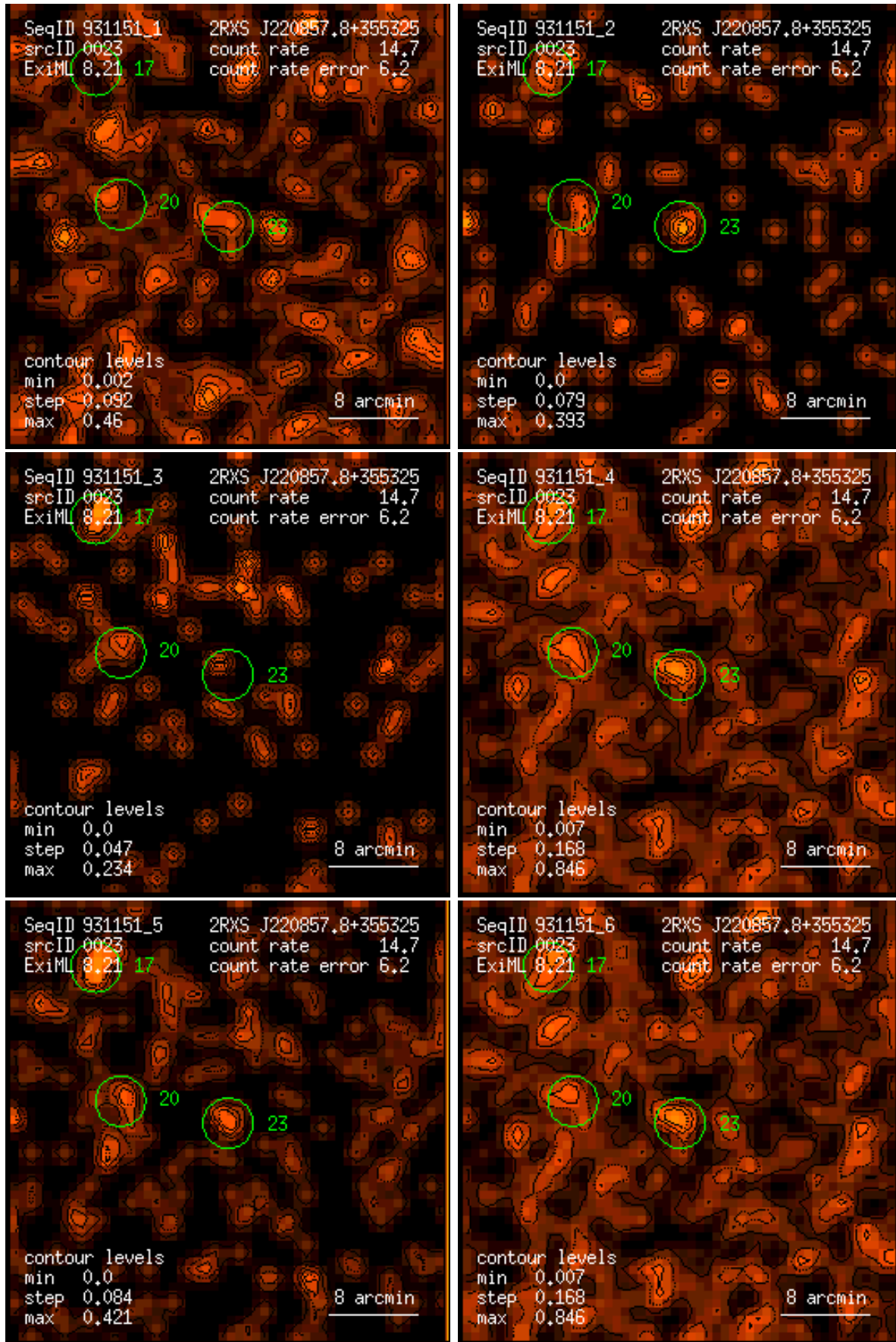
Figure 23: RASS 931151: detection 0023: band rate images, Gaussian filter: (1) PSPC channels 11 – 41, (2) 52 – 90, (3) 91 – 201, (4) 11 – 235, (5) 52 – 201, (6) 11 – 201. Broad band rates in counts/ks. Band rate contour levels in counts/ks/arcmin 2 .
