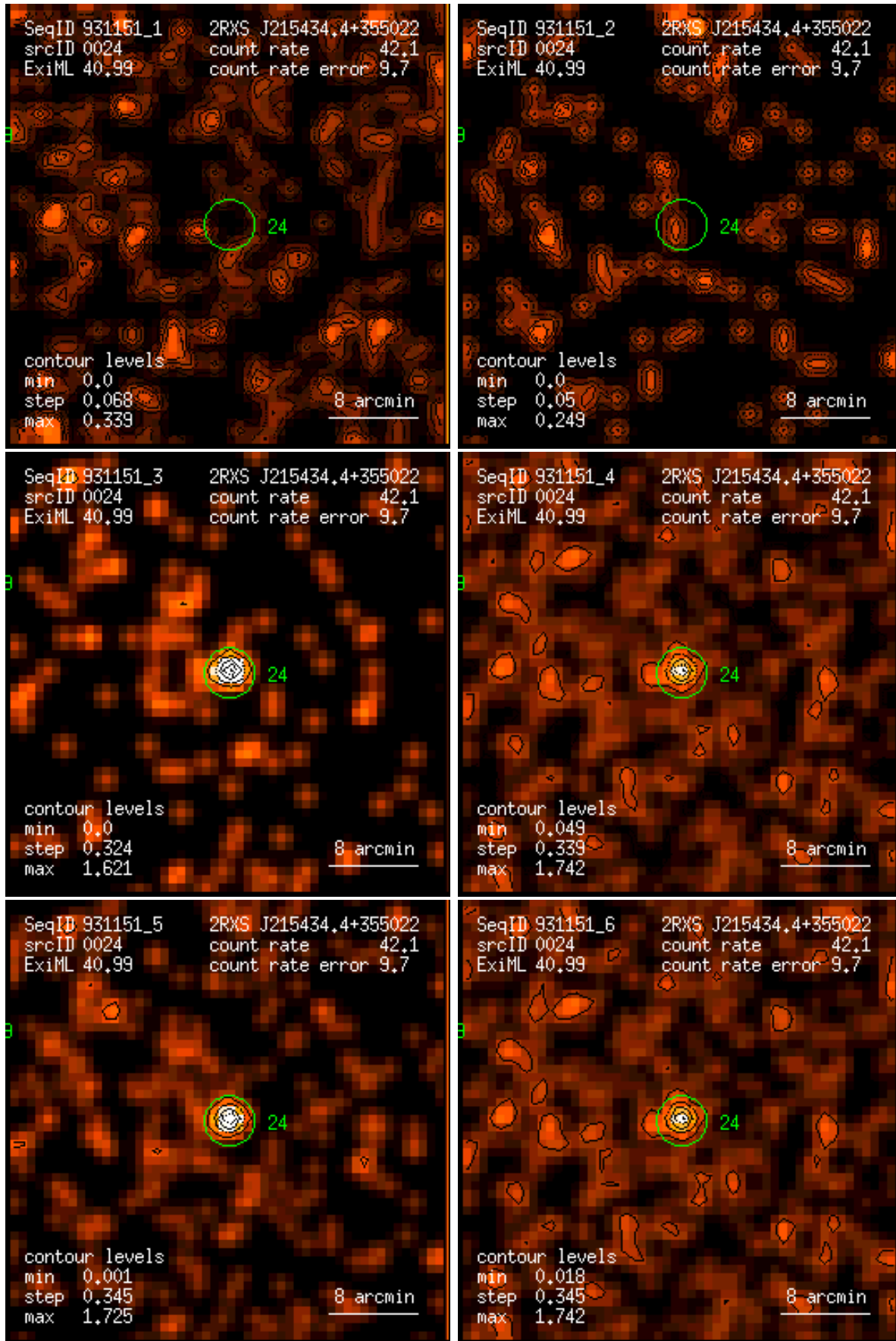
Figure 24: RASS 931151: detection 0024: band rate images, Gaussian filter: (1) PSPC channels 11 – 41, (2) 52 – 90, (3) 91 – 201, (4) 11 – 235, (5) 52 – 201, (6) 11 – 201. Broad band rates in counts/ks. Band rate contour levels in counts/ks/arcmin 2 .
