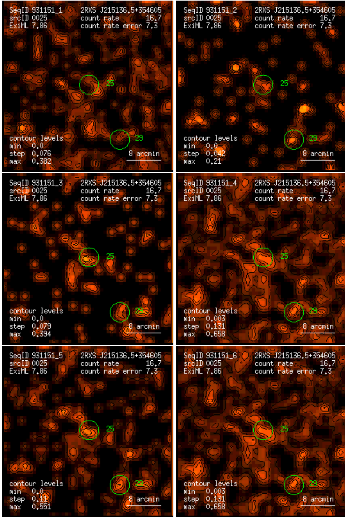
Figure 25: RASS 931151: detection 0025: band rate images, Gaussian filter: (1) PSPC channels 11 – 41, (2) 52 – 90, (3) 91 – 201, (4) 11 – 235, (5) 52 – 201, (6) 11 – 201. Broad band rates in counts/ks. Band rate contour levels in counts/ks/arcmin 2 .
