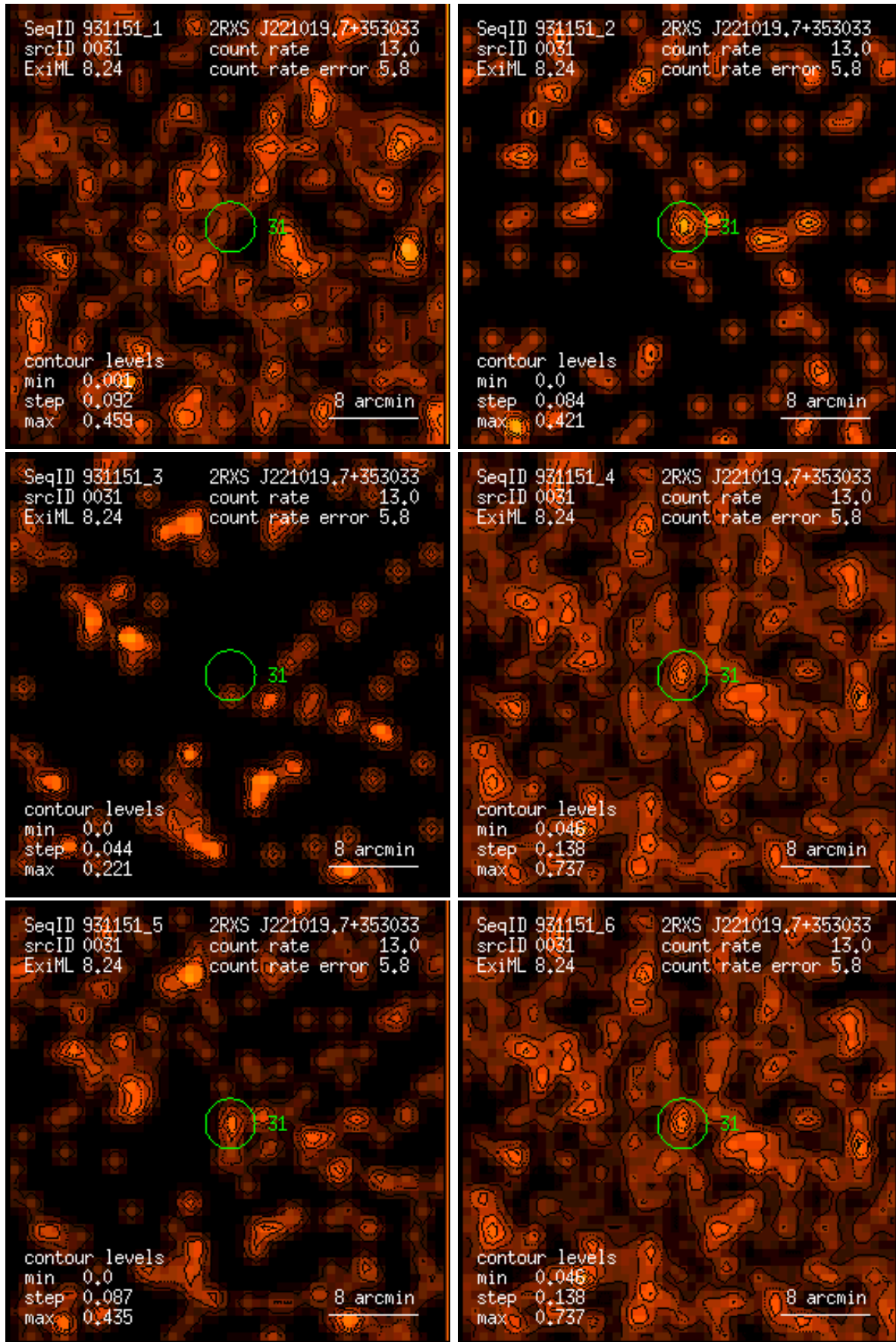
Figure 31: RASS 931151: detection 0031: band rate images, Gaussian filter: (1) PSPC channels 11 – 41, (2) 52 – 90, (3) 91 – 201, (4) 11 – 235, (5) 52 – 201, (6) 11 – 201. Broad band rates in counts/ks. Band rate contour levels in counts/ks/arcmin 2 .
