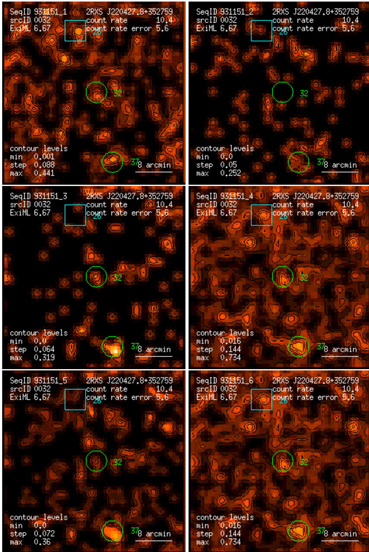
Figure 32: RASS 931151: detection 0032: band rate images, Gaussian filter: (1) PSPC channels 11 – 41, (2) 52 – 90, (3) 91 – 201, (4) 11 – 235, (5) 52 – 201, (6) 11 – 201. Broad band rates in counts/ks. Band rate contour levels in counts/ks/arcmin 2 .
