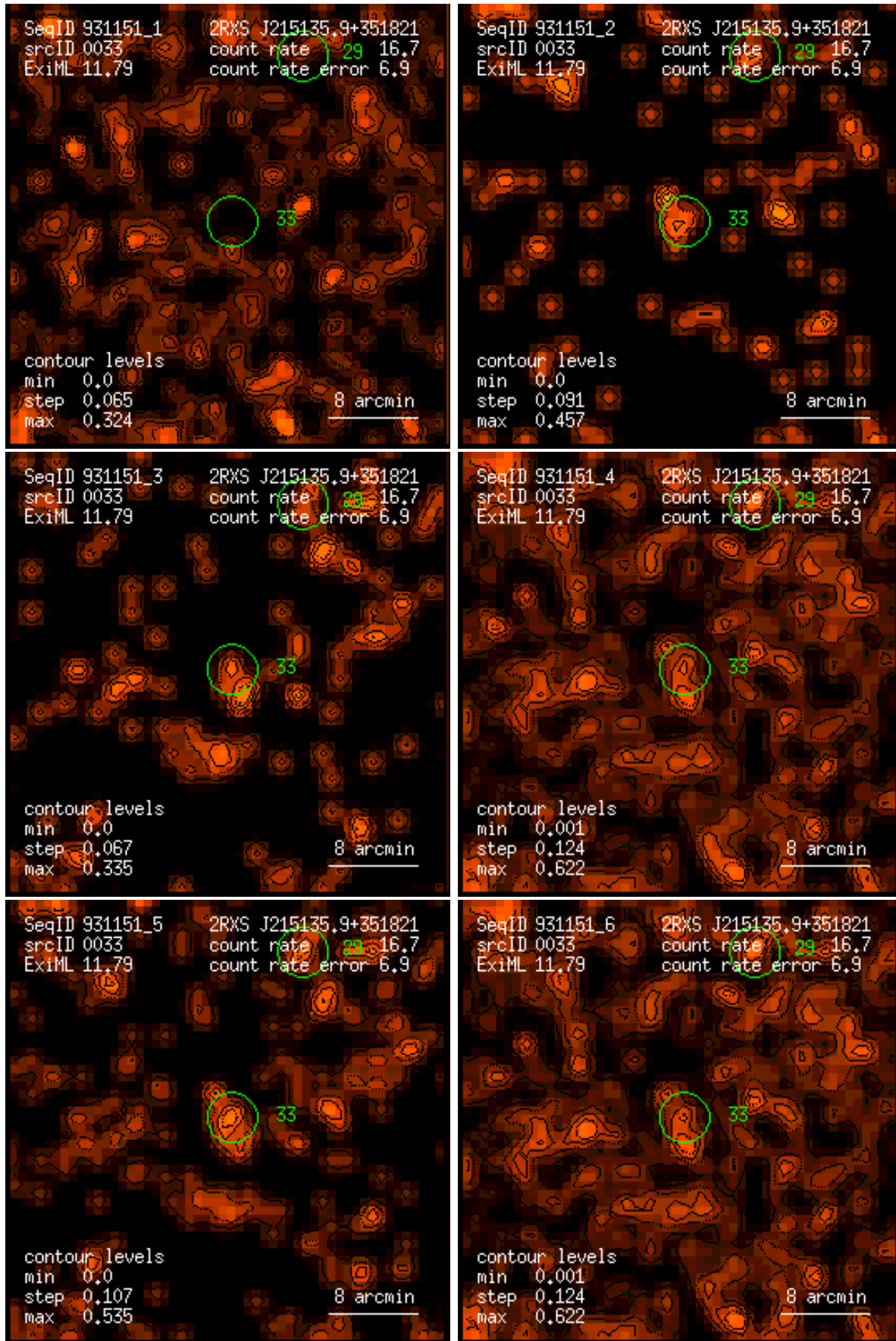
Figure 33: RASS 931151: detection 0033: band rate images, Gaussian filter: (1) PSPC channels 11 – 41, (2) 52 – 90, (3) 91 – 201, (4) 11 – 235, (5) 52 – 201, (6) 11 – 201. Broad band rates in counts/ks. Band rate contour levels in counts/ks/arcmin 2 .
