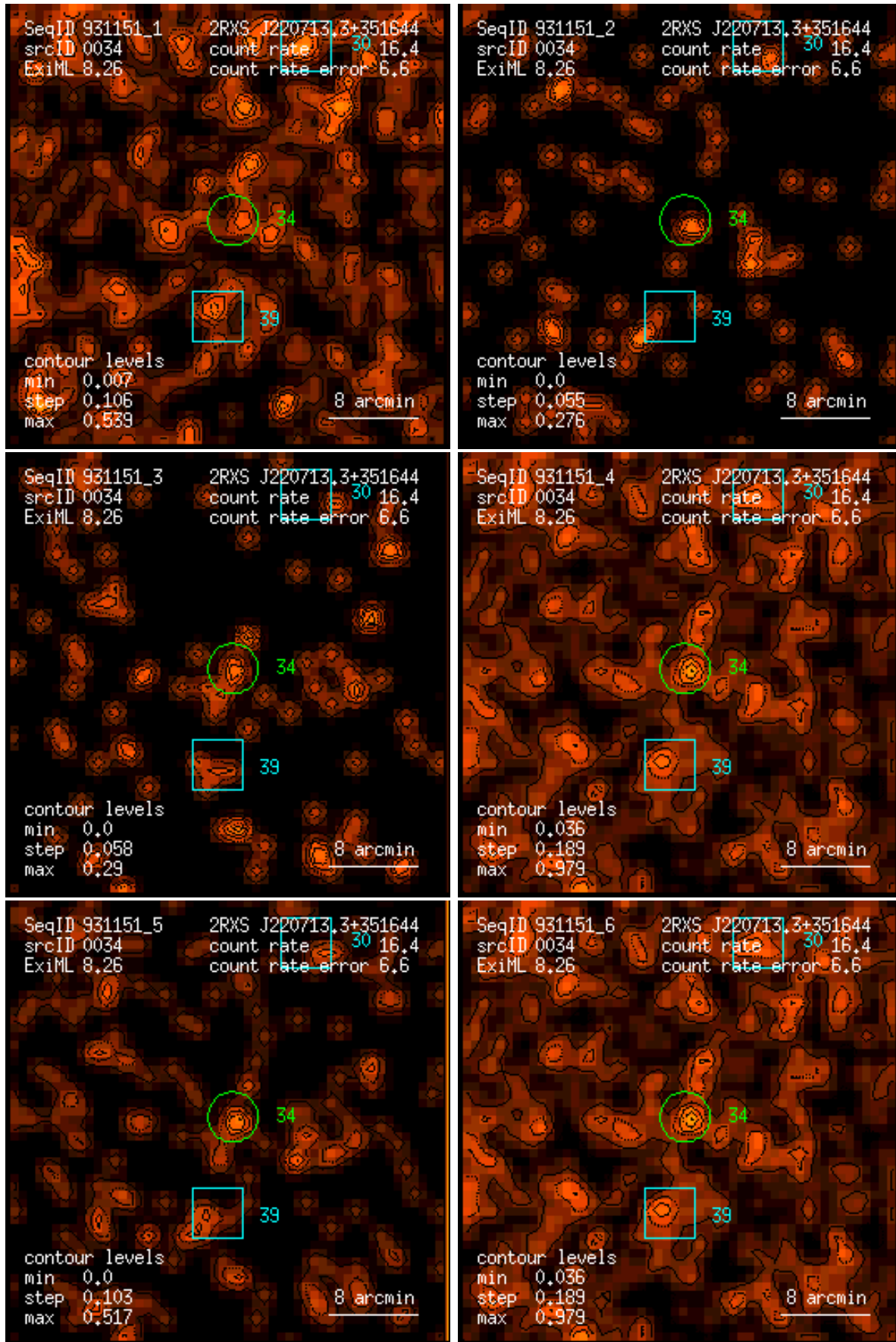
Figure 34: RASS 931151: detection 0034: band rate images, Gaussian filter: (1) PSPC channels 11 – 41, (2) 52 – 90, (3) 91 – 201, (4) 11 – 235, (5) 52 – 201, (6) 11 – 201. Broad band rates in counts/ks. Band rate contour levels in counts/ks/arcmin 2 .
