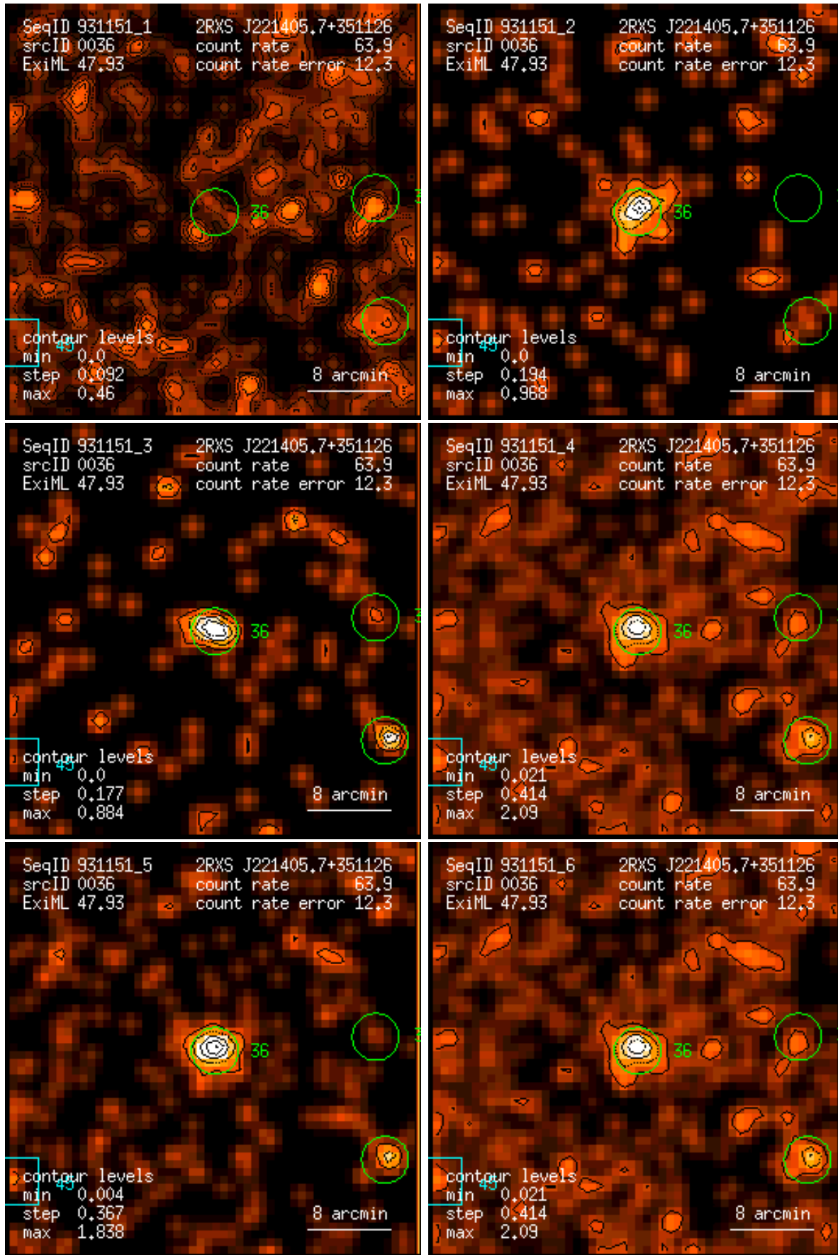
Figure 36: RASS 931151: detection 0036: band rate images, Gaussian filter: (1) PSPC channels 11 – 41, (2) 52 – 90, (3) 91 – 201, (4) 11 – 235, (5) 52 – 201, (6) 11 – 201. Broad band rates in counts/ks. Band rate contour levels in counts/ks/arcmin 2 .
