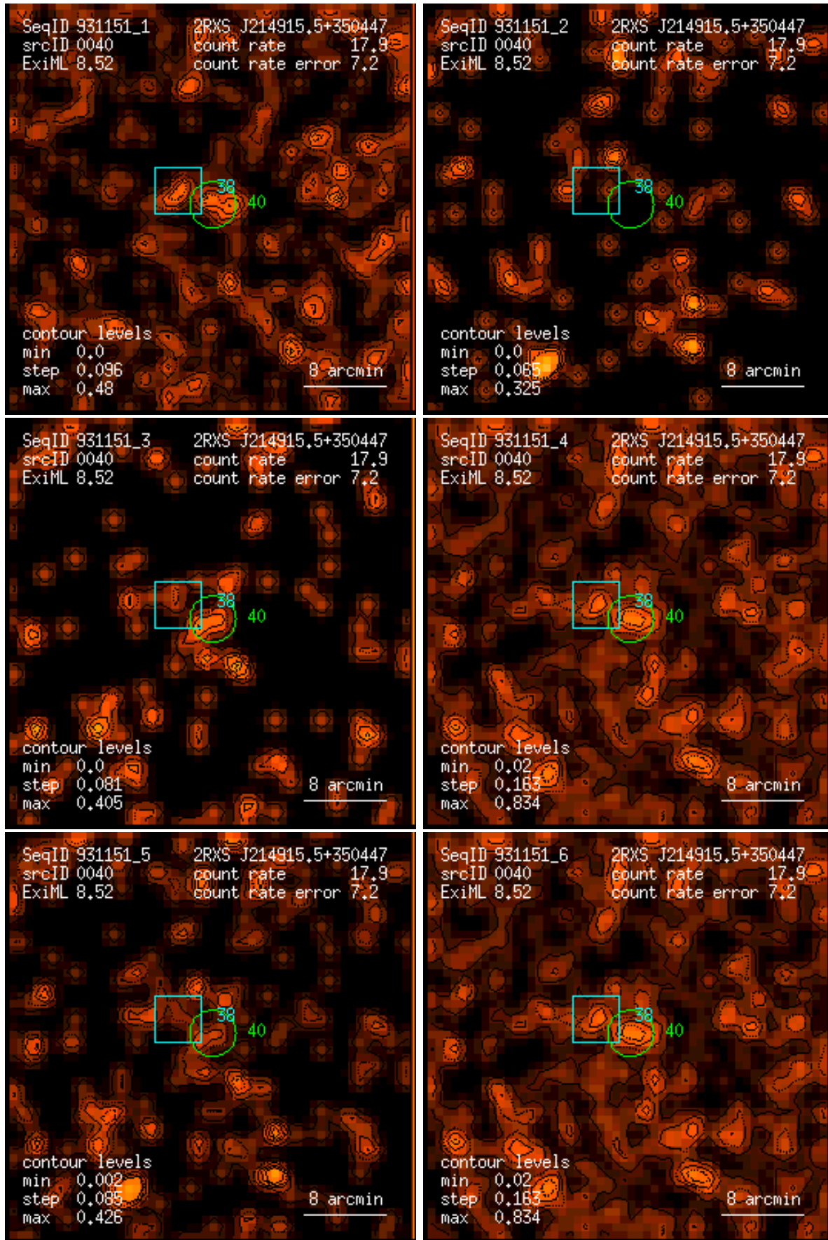
Figure 40: RASS 931151: detection 0040: band rate images, Gaussian filter: (1) PSPC channels 11 – 41, (2) 52 – 90, (3) 91 – 201, (4) 11 – 235, (5) 52 – 201, (6) 11 – 201. Broad band rates in counts/ks. Band rate contour levels in counts/ks/arcmin 2 .
