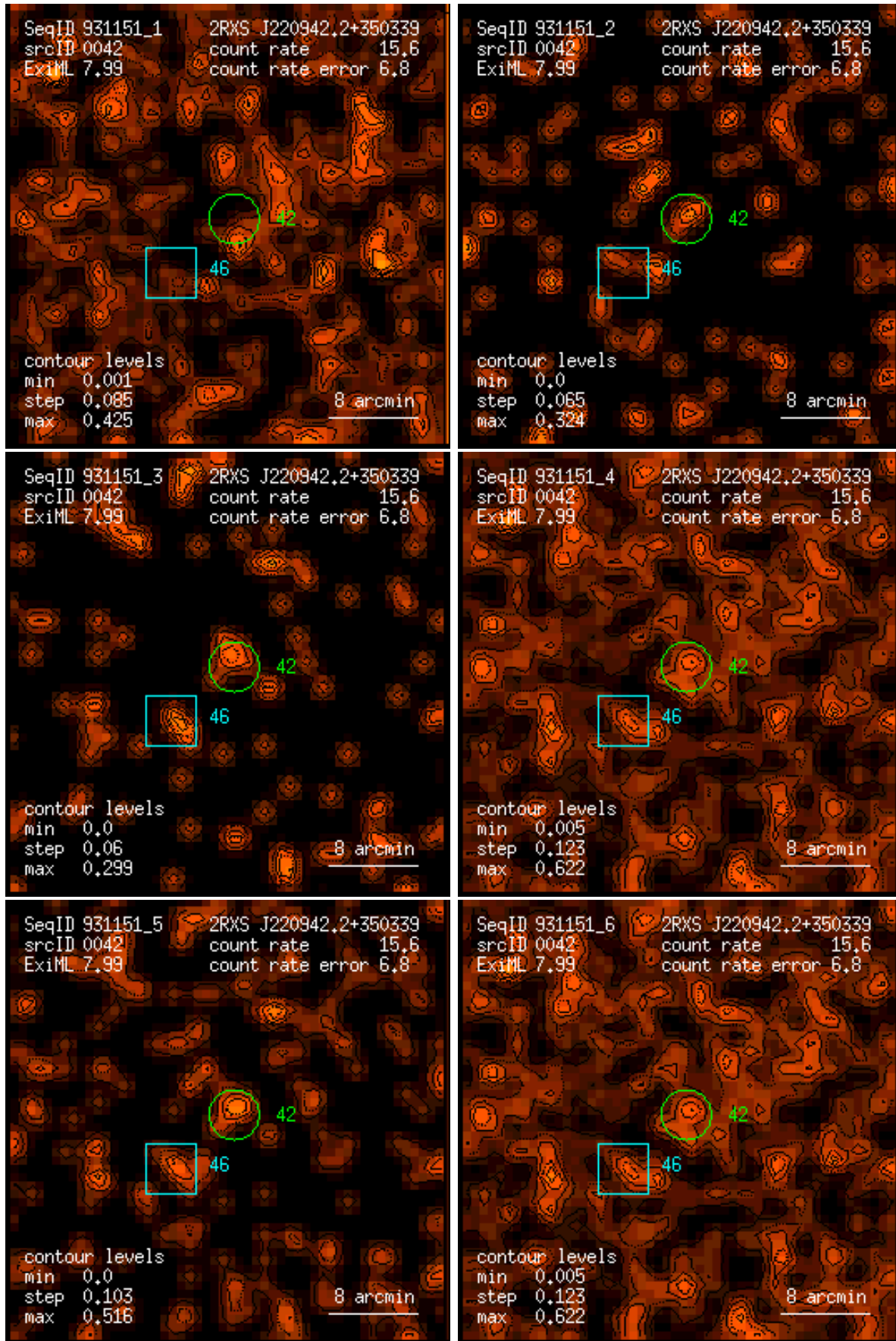
Figure 42: RASS 931151: detection 0042: band rate images, Gaussian filter: (1) PSPC channels 11 – 41, (2) 52 – 90, (3) 91 – 201, (4) 11 – 235, (5) 52 – 201, (6) 11 – 201. Broad band rates in counts/ks. Band rate contour levels in counts/ks/arcmin 2 .
