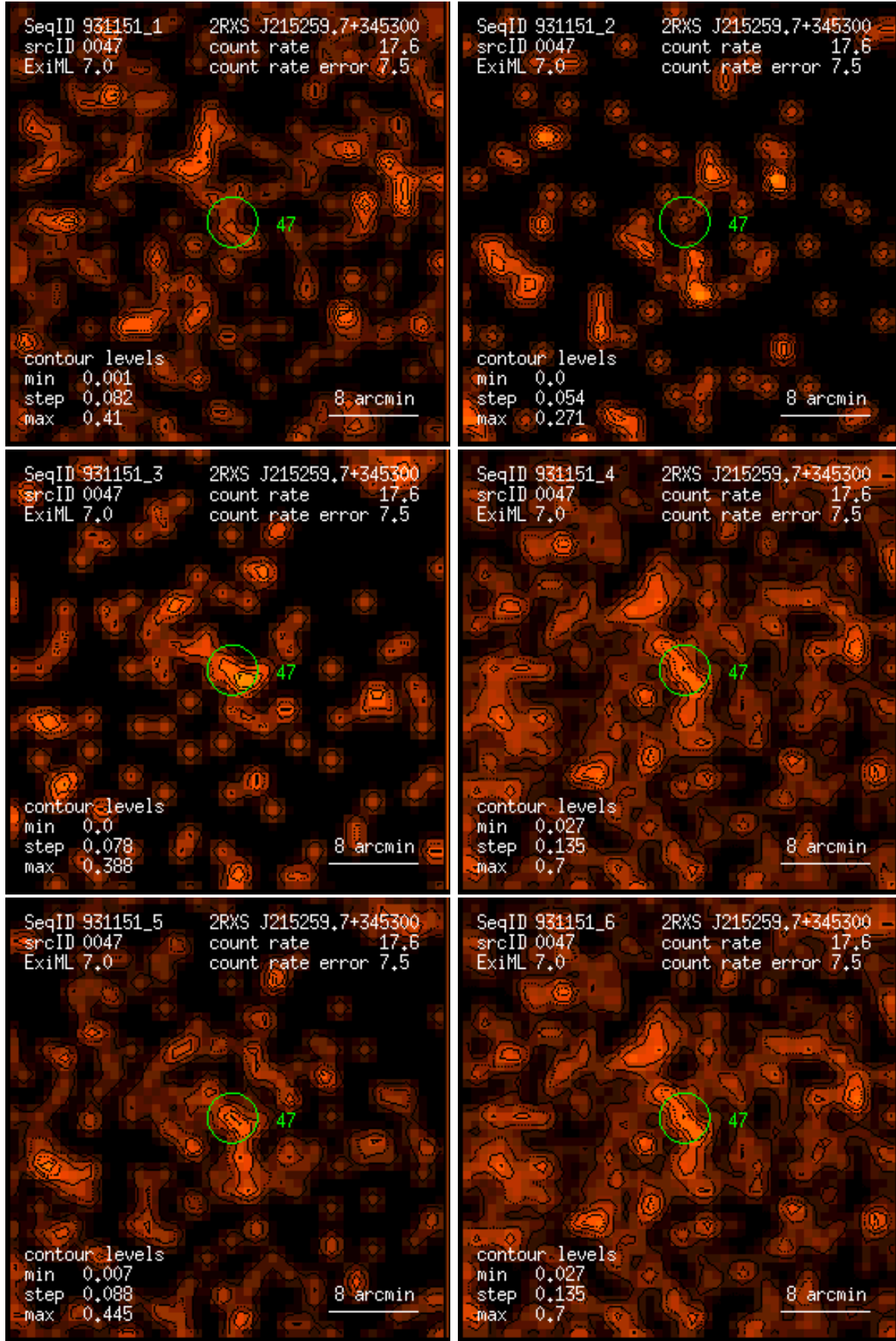
Figure 47: RASS 931151: detection 0047: band rate images, Gaussian filter: (1) PSPC channels 11 – 41, (2) 52 – 90, (3) 91 – 201, (4) 11 – 235, (5) 52 – 201, (6) 11 – 201. Broad band rates in counts/ks. Band rate contour levels in counts/ks/arcmin 2 .
