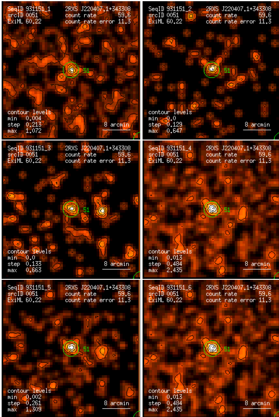
Figure 51: RASS 931151: detection 0051: band rate images, Gaussian filter: (1) PSPC channels 11 – 41, (2) 52 – 90, (3) 91 – 201, (4) 11 – 235, (5) 52 – 201, (6) 11 – 201. Broad band rates in counts/ks. Band rate contour levels in counts/ks/arcmin 2 .
