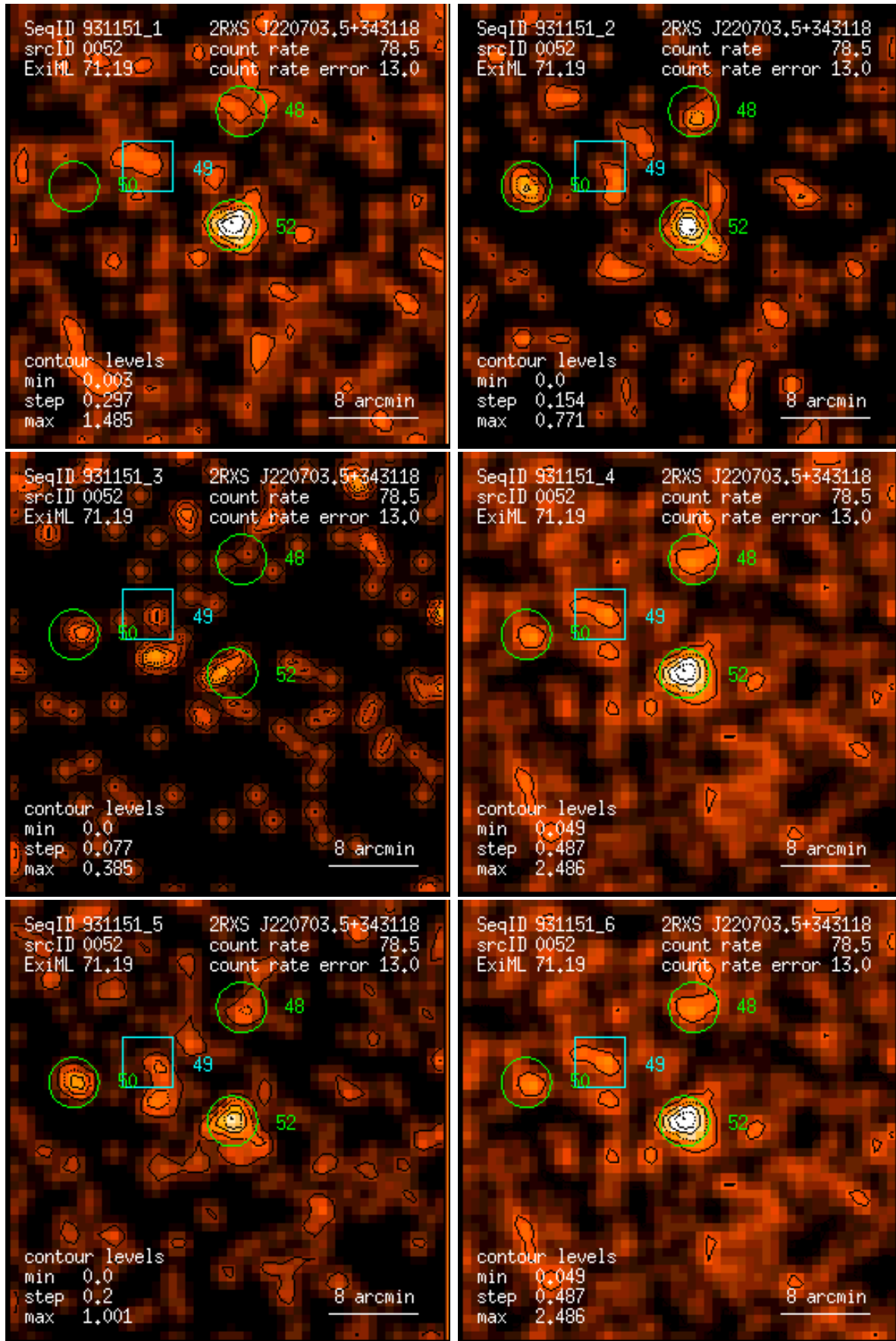
Figure 52: RASS 931151: detection 0052: band rate images, Gaussian filter: (1) PSPC channels 11 – 41, (2) 52 – 90, (3) 91 – 201, (4) 11 – 235, (5) 52 – 201, (6) 11 – 201. Broad band rates in counts/ks. Band rate contour levels in counts/ks/arcmin 2 .
