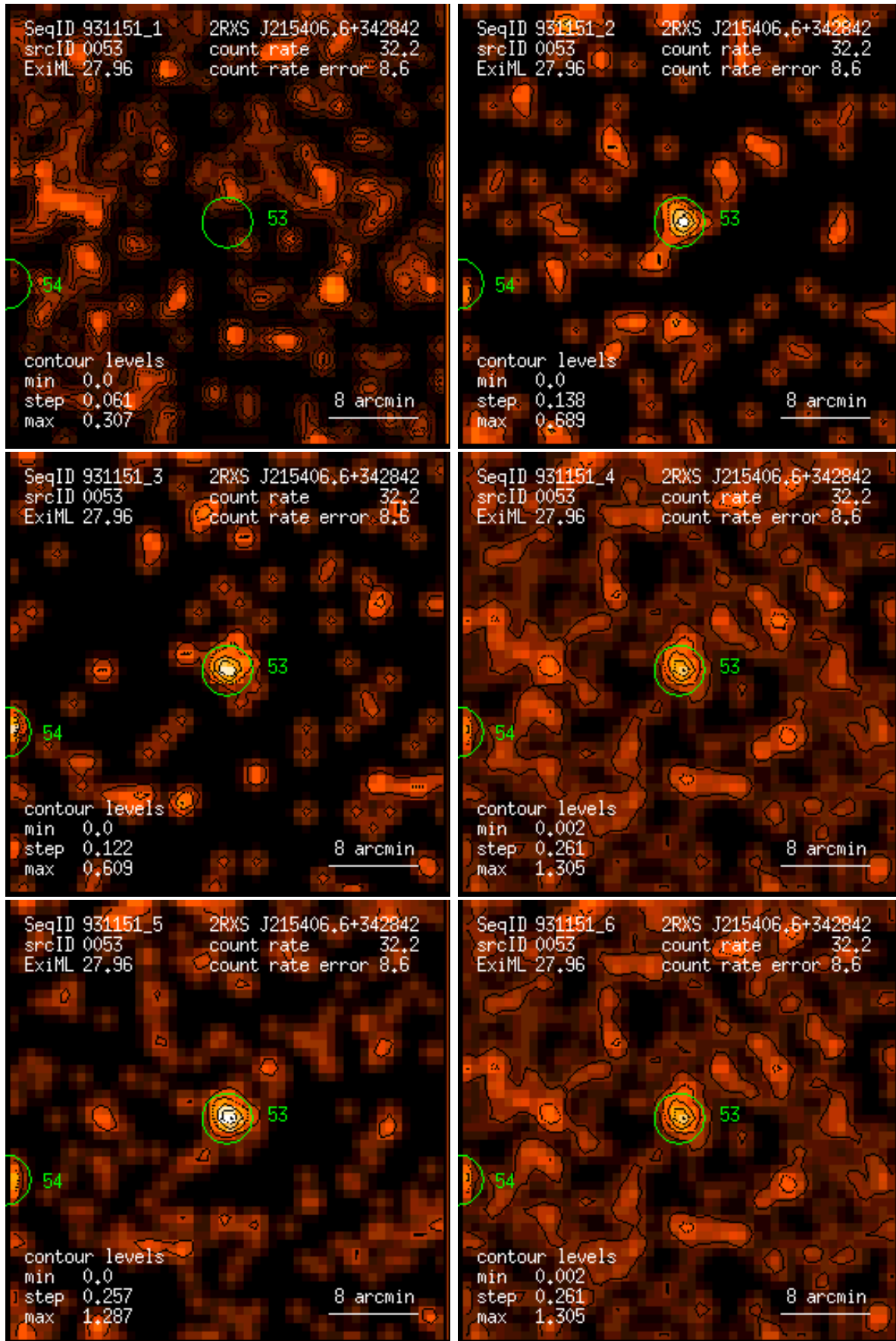
Figure 53: RASS 931151: detection 0053: band rate images, Gaussian filter: (1) PSPC channels 11 – 41, (2) 52 – 90, (3) 91 – 201, (4) 11 – 235, (5) 52 – 201, (6) 11 – 201. Broad band rates in counts/ks. Band rate contour levels in counts/ks/arcmin 2 .
