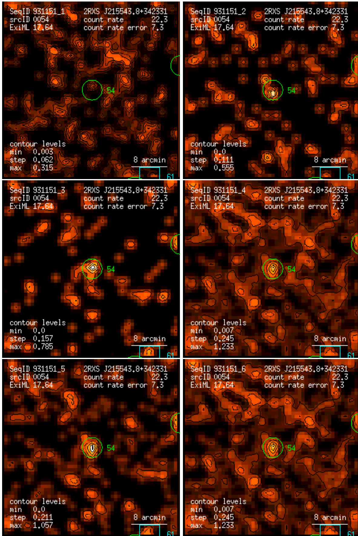
Figure 54: RASS 931151: detection 0054: band rate images, Gaussian filter: (1) PSPC channels 11 – 41, (2) 52 – 90, (3) 91 – 201, (4) 11 – 235, (5) 52 – 201, (6) 11 – 201. Broad band rates in counts/ks. Band rate contour levels in counts/ks/arcmin 2 .
