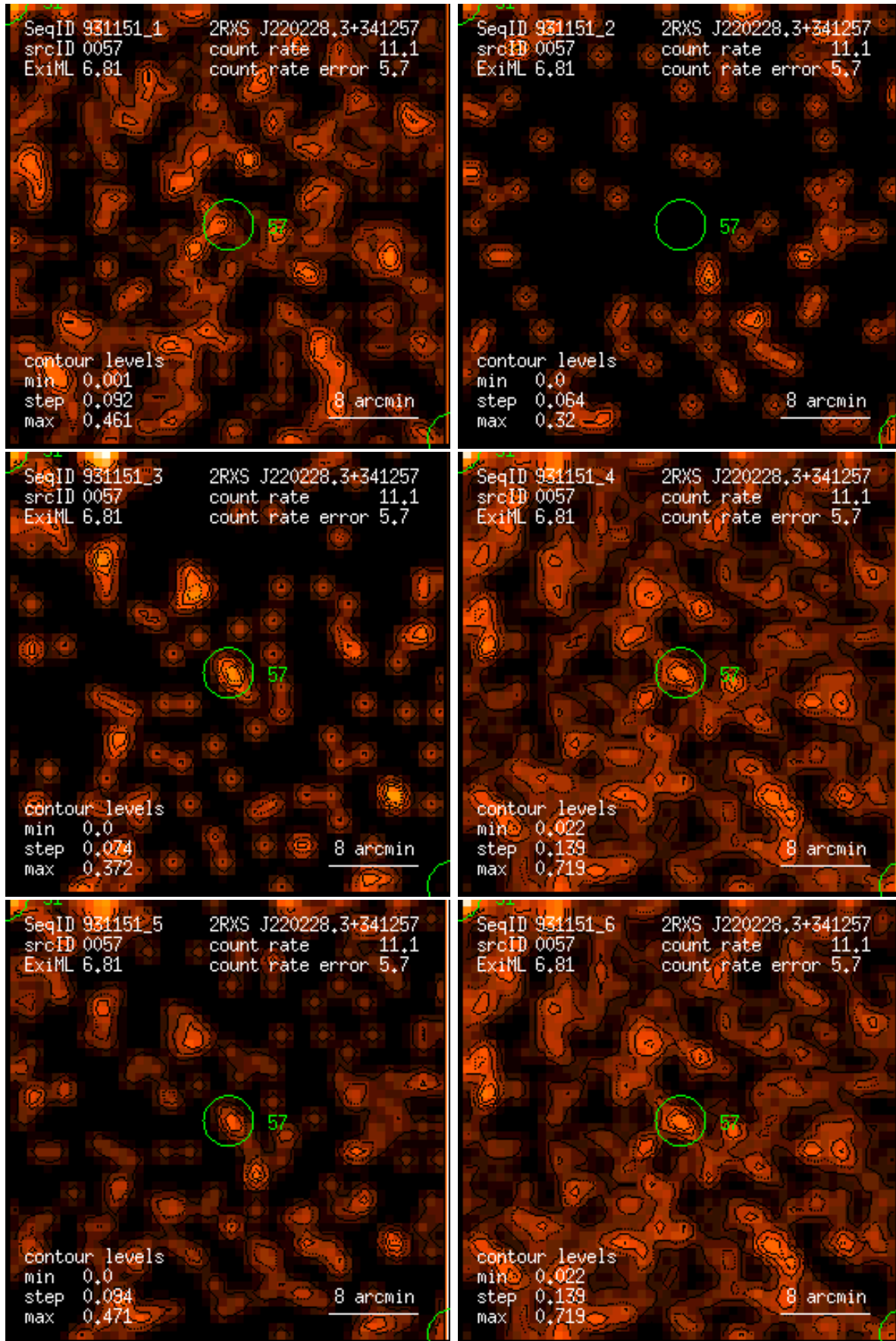
Figure 57: RASS 931151: detection 0057: band rate images, Gaussian filter: (1) PSPC channels 11 – 41, (2) 52 – 90, (3) 91 – 201, (4) 11 – 235, (5) 52 – 201, (6) 11 – 201. Broad band rates in counts/ks. Band rate contour levels in counts/ks/arcmin 2 .
