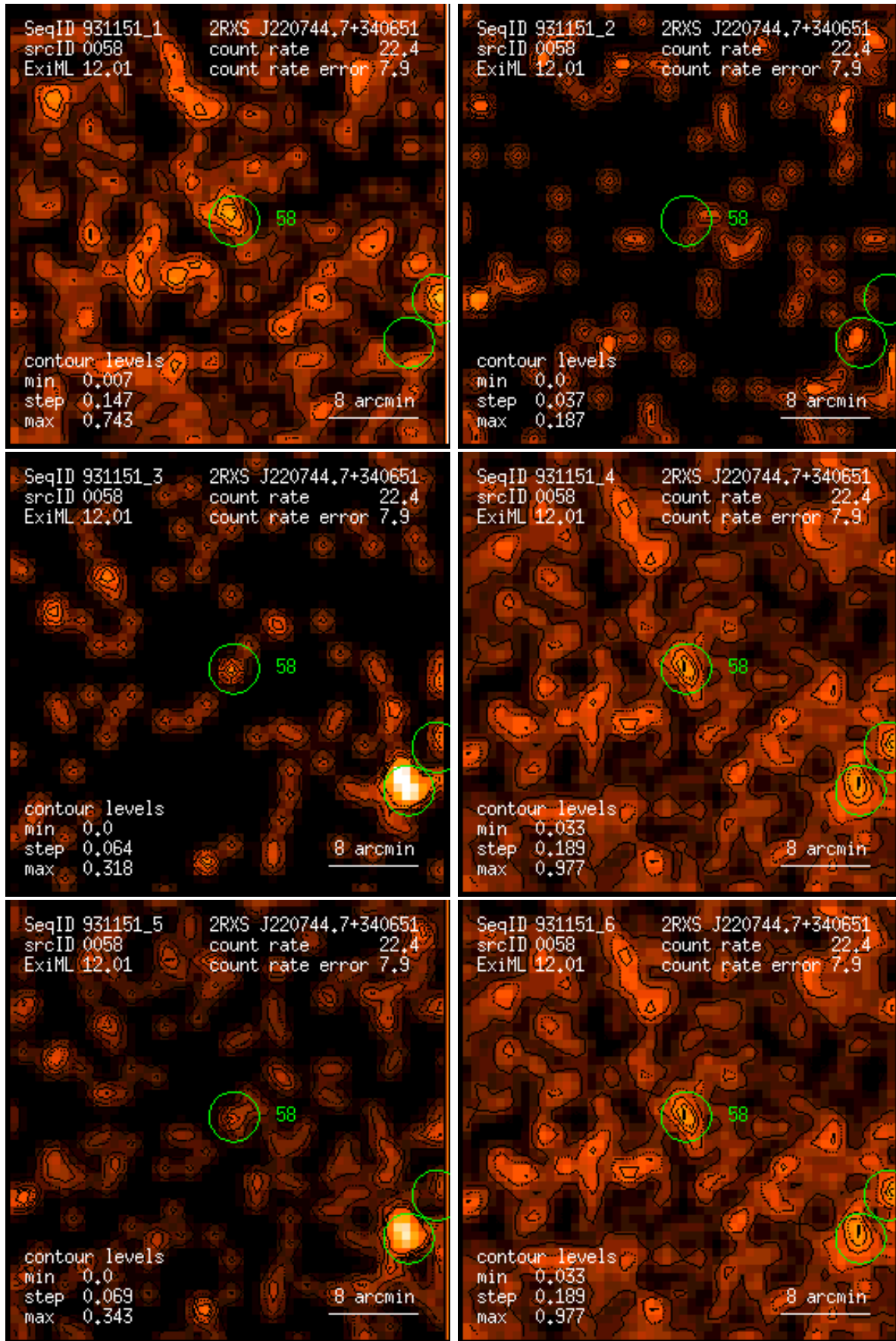
Figure 58: RASS 931151: detection 0058: band rate images, Gaussian filter: (1) PSPC channels 11 – 41, (2) 52 – 90, (3) 91 – 201, (4) 11 – 235, (5) 52 – 201, (6) 11 – 201. Broad band rates in counts/ks. Band rate contour levels in counts/ks/arcmin 2 .
