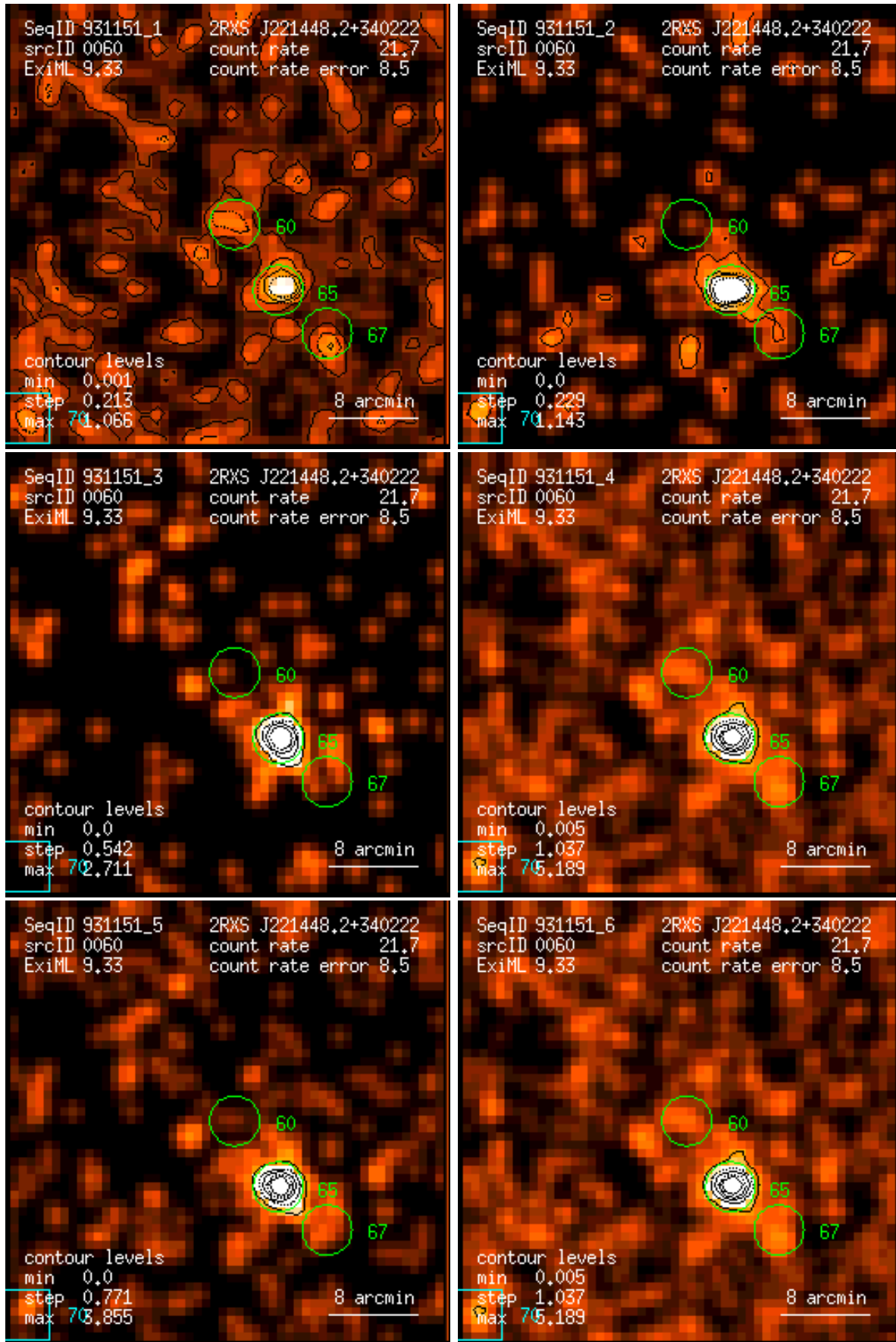
Figure 60: RASS 931151: detection 0060: band rate images, Gaussian filter: (1) PSPC channels 11 – 41, (2) 52 – 90, (3) 91 – 201, (4) 11 – 235, (5) 52 – 201, (6) 11 – 201. Broad band rates in counts/ks. Band rate contour levels in counts/ks/arcmin 2 .
