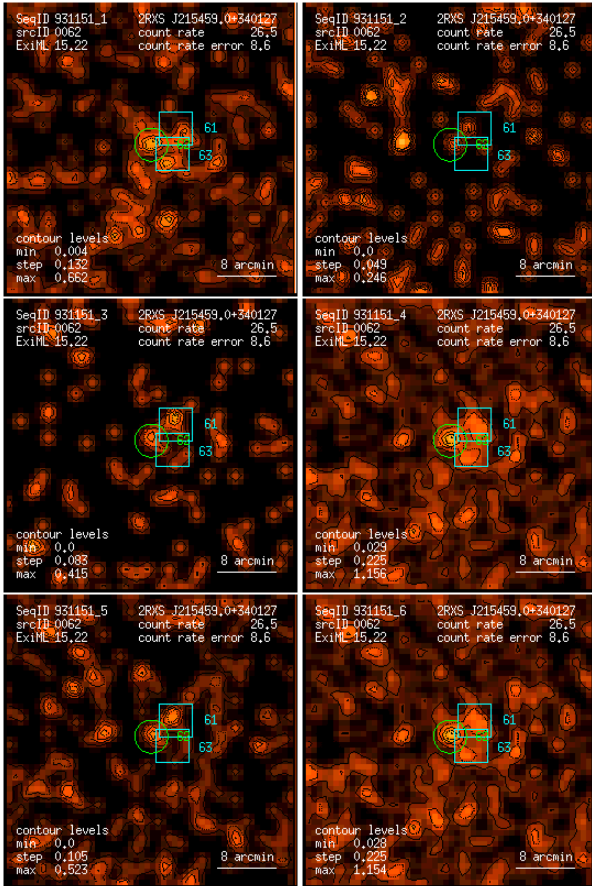
Figure 62: RASS 931151: detection 0062: band rate images, Gaussian filter: (1) PSPC channels 11 – 41, (2) 52 – 90, (3) 91 – 201, (4) 11 – 235, (5) 52 – 201, (6) 11 – 201. Broad band rates in counts/ks. Band rate contour levels in counts/ks/arcmin 2 .
