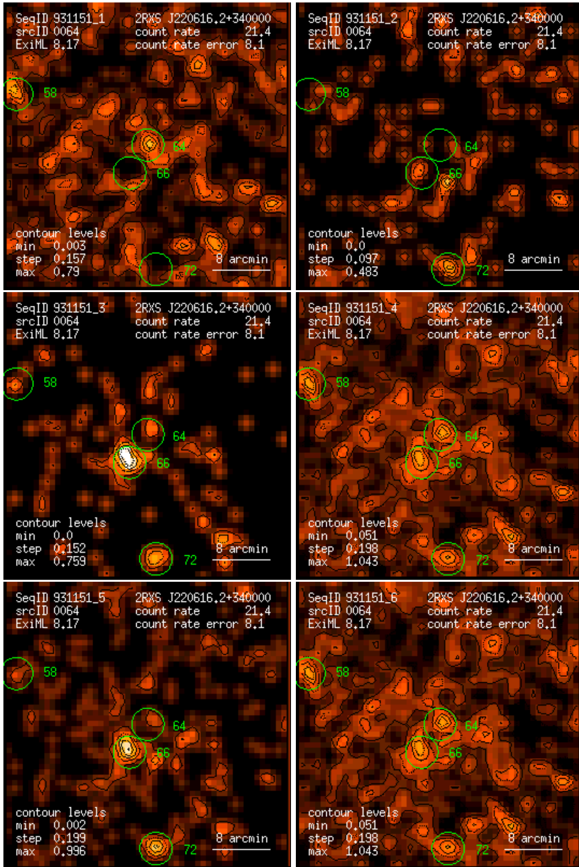
Figure 64: RASS 931151: detection 0064: band rate images, Gaussian filter: (1) PSPC channels 11 – 41, (2) 52 – 90, (3) 91 – 201, (4) 11 – 235, (5) 52 – 201, (6) 11 – 201. Broad band rates in counts/ks. Band rate contour levels in counts/ks/arcmin 2 .
