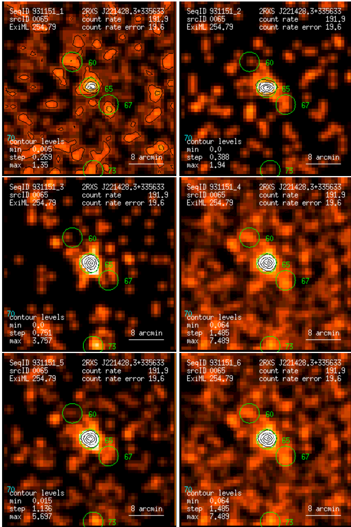
Figure 65: RASS 931151: detection 0065: band rate images, Gaussian filter: (1) PSPC channels 11 – 41, (2) 52 – 90, (3) 91 – 201, (4) 11 – 235, (5) 52 – 201, (6) 11 – 201. Broad band rates in counts/ks. Band rate contour levels in counts/ks/arcmin 2 .
