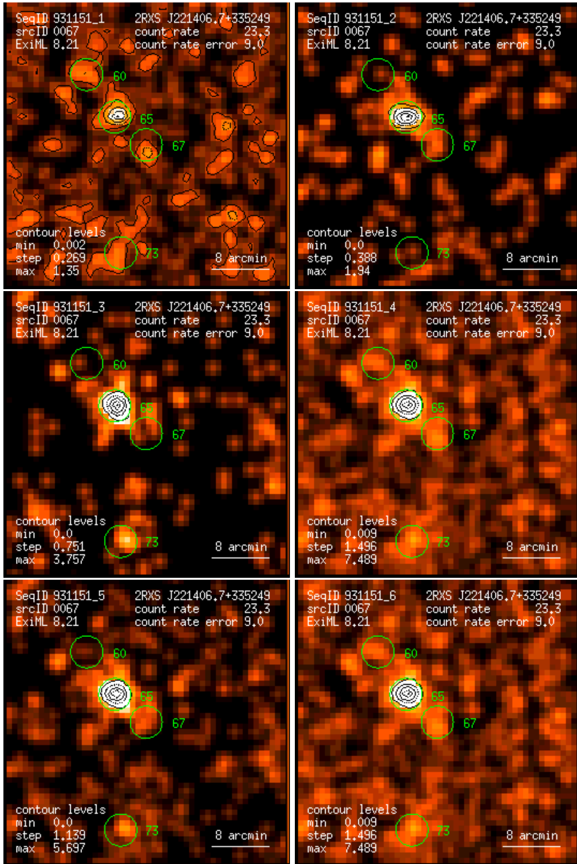
Figure 67: RASS 931151: detection 0067: band rate images, Gaussian filter: (1) PSPC channels 11 – 41, (2) 52 – 90, (3) 91 – 201, (4) 11 – 235, (5) 52 – 201, (6) 11 – 201. Broad band rates in counts/ks. Band rate contour levels in counts/ks/arcmin 2 .
