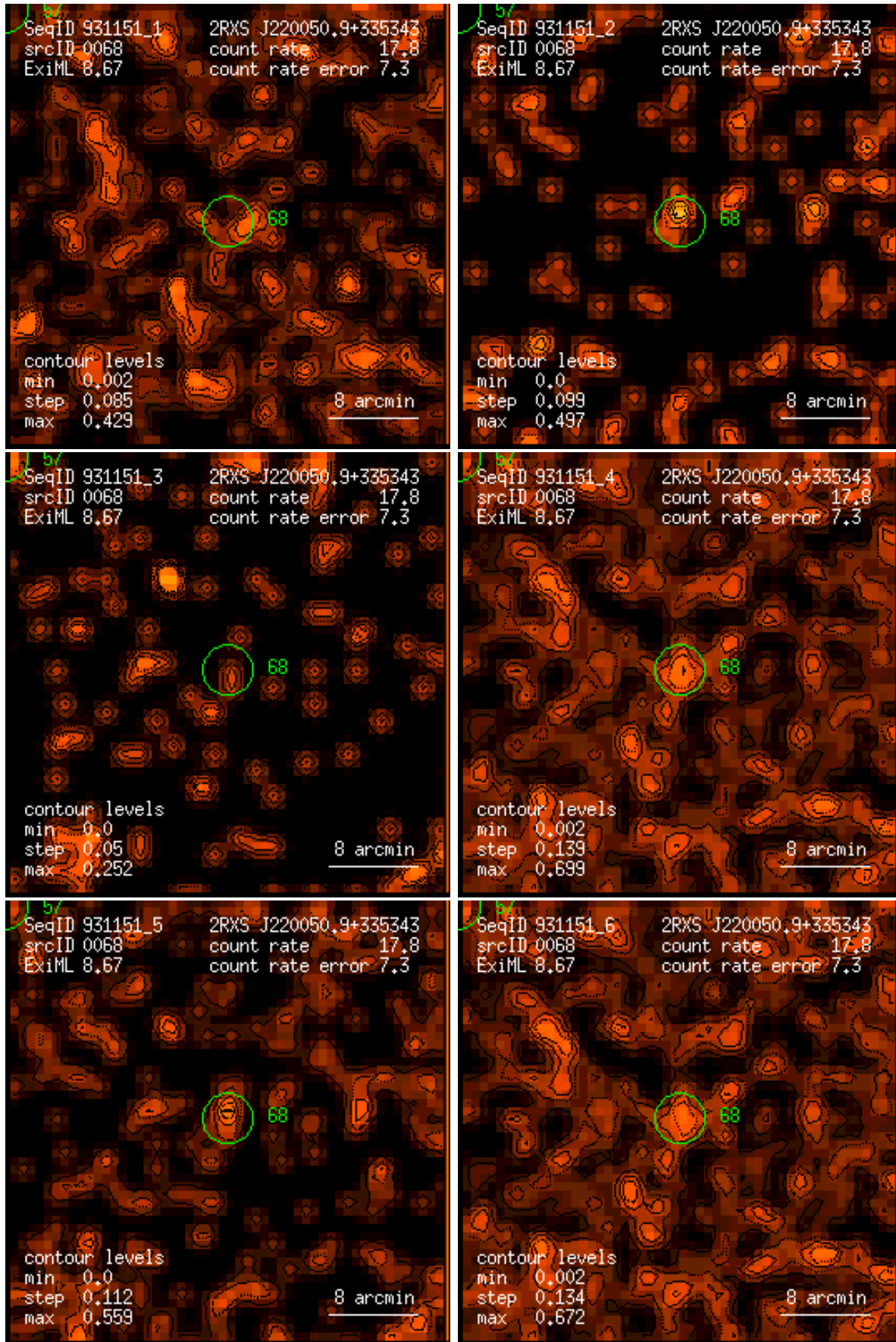
Figure 68: RASS 931151: detection 0068: band rate images, Gaussian filter: (1) PSPC channels 11 – 41, (2) 52 – 90, (3) 91 – 201, (4) 11 – 235, (5) 52 – 201, (6) 11 – 201. Broad band rates in counts/ks. Band rate contour levels in counts/ks/arcmin 2 .
