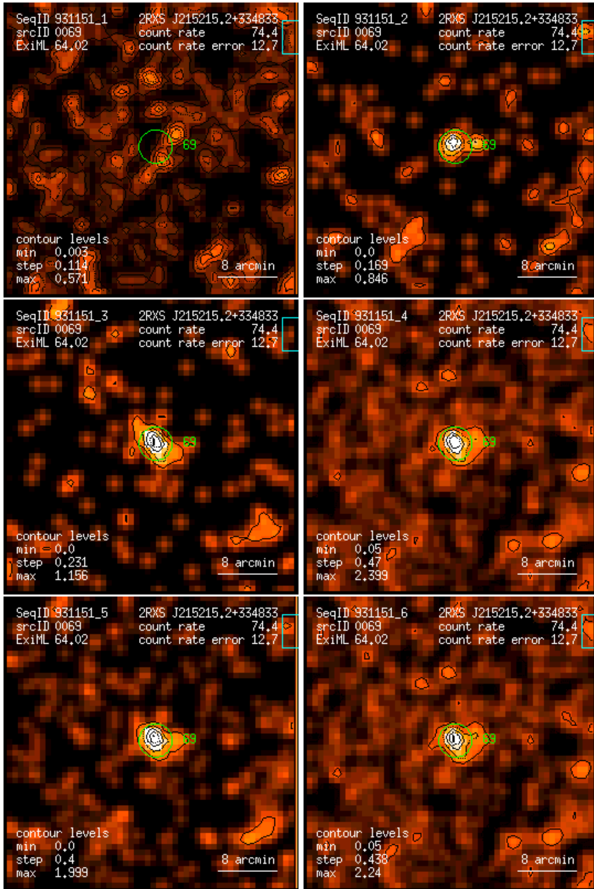
Figure 69: RASS 931151: detection 0069: band rate images, Gaussian filter: (1) PSPC channels 11 – 41, (2) 52 – 90, (3) 91 – 201, (4) 11 – 235, (5) 52 – 201, (6) 11 – 201. Broad band rates in counts/ks. Band rate contour levels in counts/ks/arcmin 2 .
