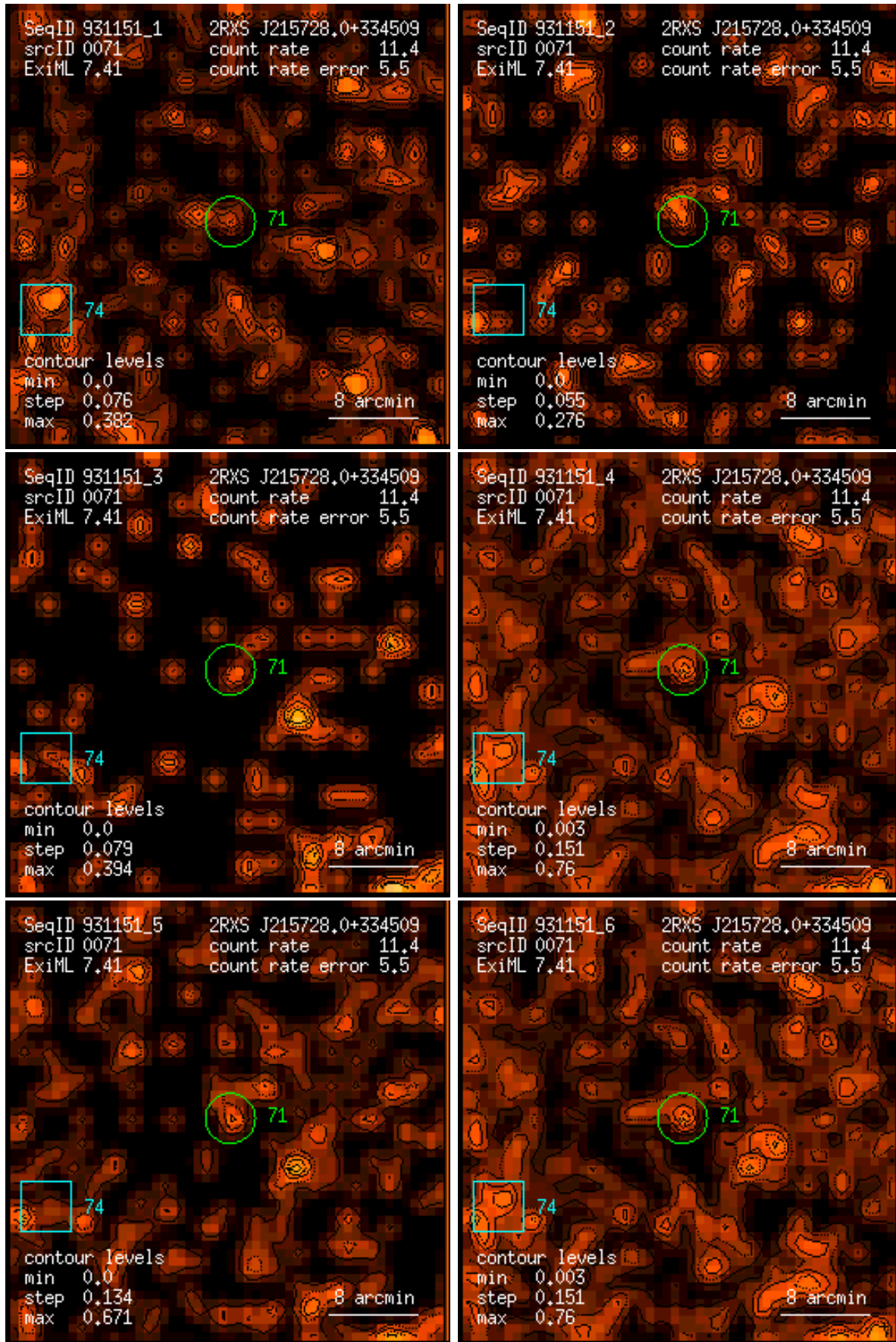
Figure 71: RASS 931151: detection 0071: band rate images, Gaussian filter: (1) PSPC channels 11 – 41, (2) 52 – 90, (3) 91 – 201, (4) 11 – 235, (5) 52 – 201, (6) 11 – 201. Broad band rates in counts/ks. Band rate contour levels in counts/ks/arcmin 2 .
