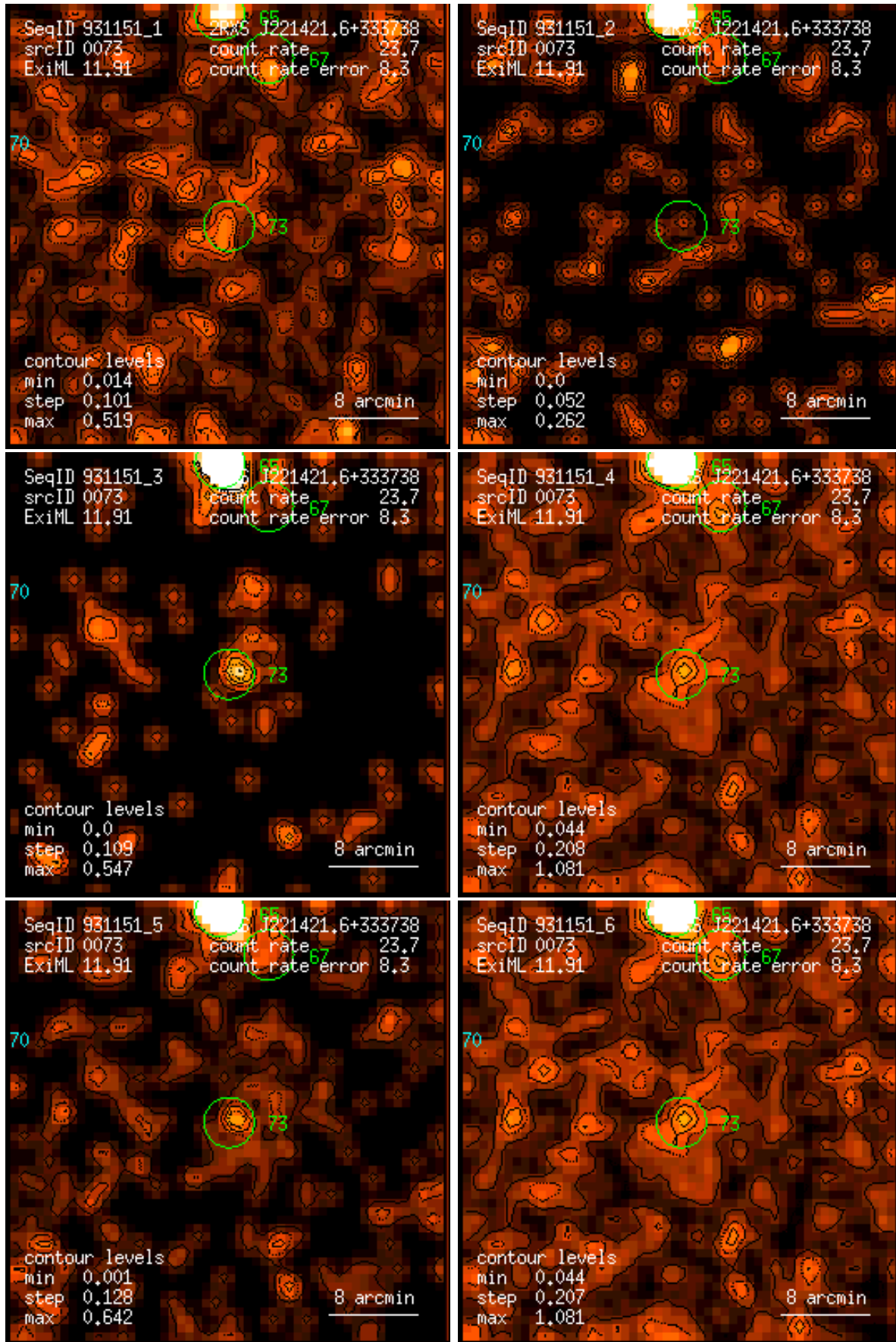
Figure 73: RASS 931151: detection 0073: band rate images, Gaussian filter: (1) PSPC channels 11 – 41, (2) 52 – 90, (3) 91 – 201, (4) 11 – 235, (5) 52 – 201, (6) 11 – 201. Broad band rates in counts/ks. Band rate contour levels in counts/ks/arcmin 2 .
