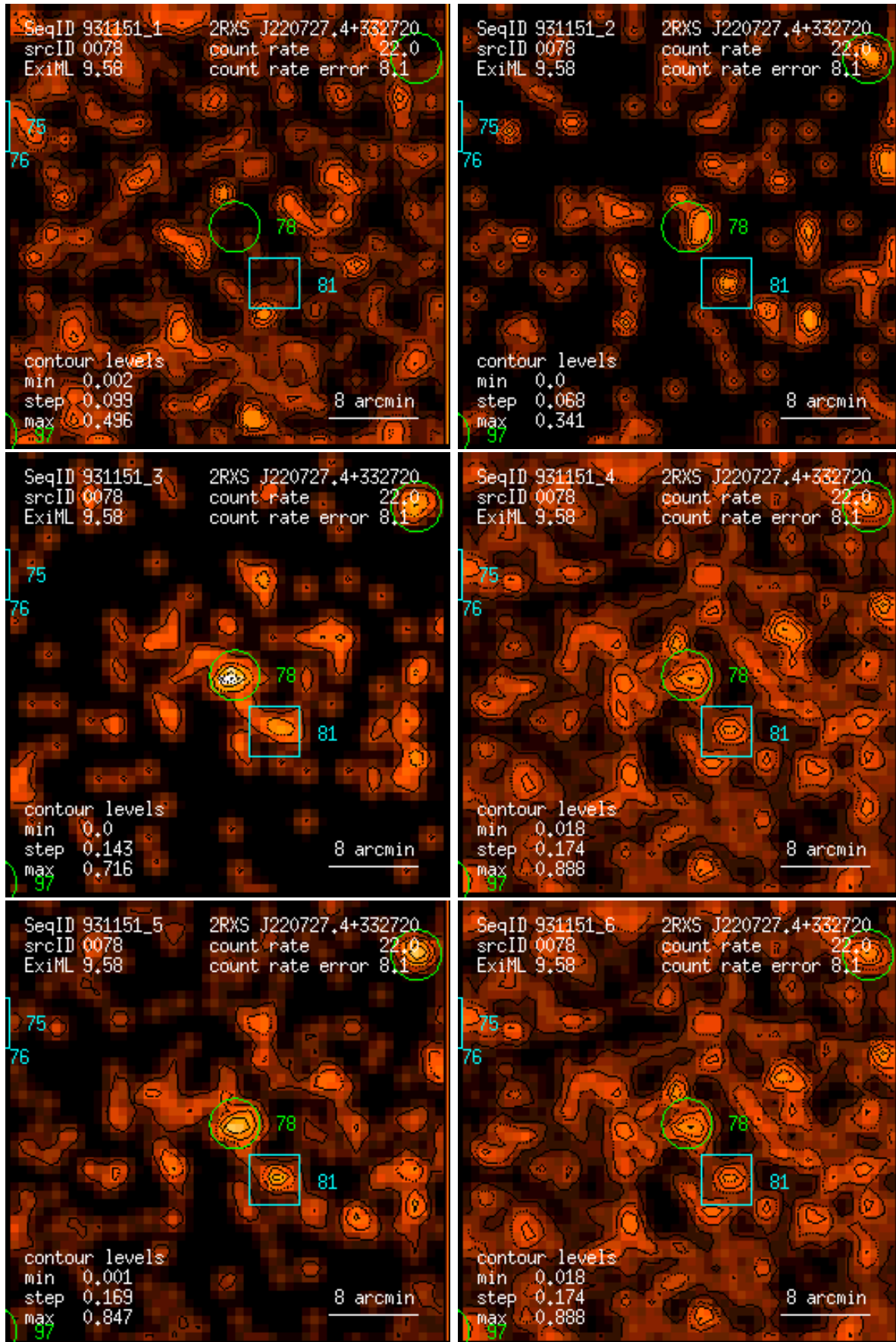
Figure 78: RASS 931151: detection 0078: band rate images, Gaussian filter: (1) PSPC channels 11 – 41, (2) 52 – 90, (3) 91 – 201, (4) 11 – 235, (5) 52 – 201, (6) 11 – 201. Broad band rates in counts/ks. Band rate contour levels in counts/ks/arcmin 2 .
