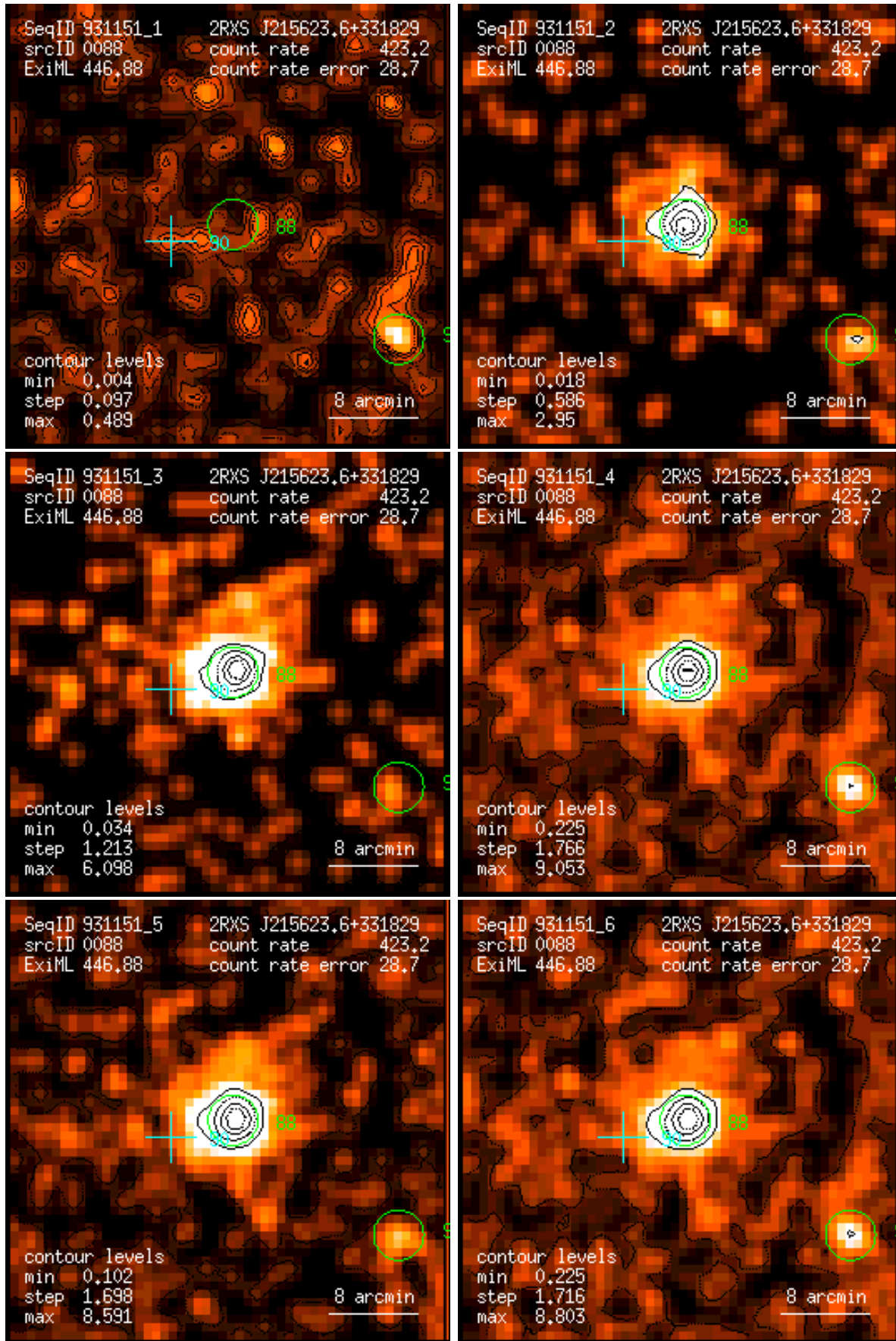
Figure 88: RASS 931151: detection 0088: band rate images, Gaussian filter: (1) PSPC channels 11 – 41, (2) 52 – 90, (3) 91 – 201, (4) 11 – 235, (5) 52 – 201, (6) 11 – 201. Broad band rates in counts/ks. Band rate contour levels in counts/ks/arcmin 2 .
