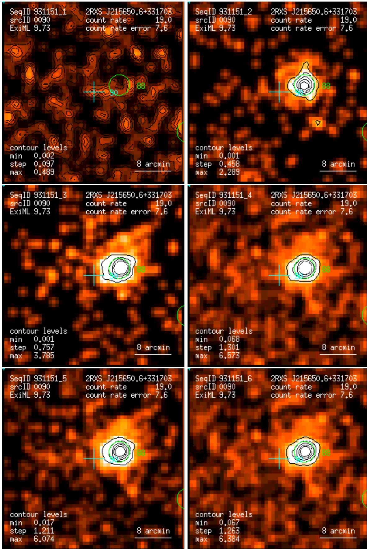
Figure 90: RASS 931151: detection 0090: band rate images, Gaussian filter: (1) PSPC channels 11 – 41, (2) 52 – 90, (3) 91 – 201, (4) 11 – 235, (5) 52 – 201, (6) 11 – 201. Broad band rates in counts/ks. Band rate contour levels in counts/ks/arcmin 2 .
