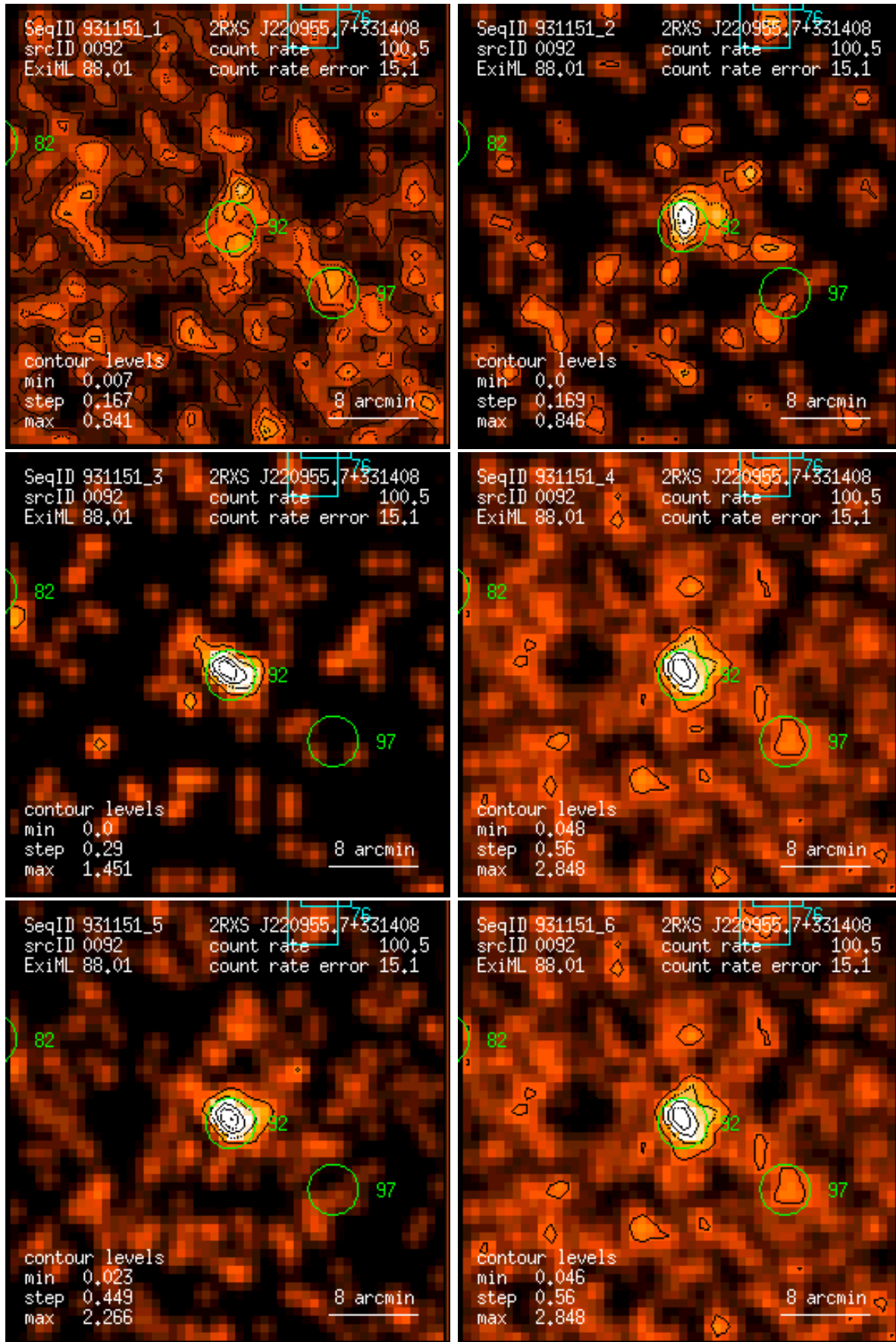
Figure 92: RASS 931151: detection 0092: band rate images, Gaussian filter: (1) PSPC channels 11 – 41, (2) 52 – 90, (3) 91 – 201, (4) 11 – 235, (5) 52 – 201, (6) 11 – 201. Broad band rates in counts/ks. Band rate contour levels in counts/ks/arcmin 2 .
