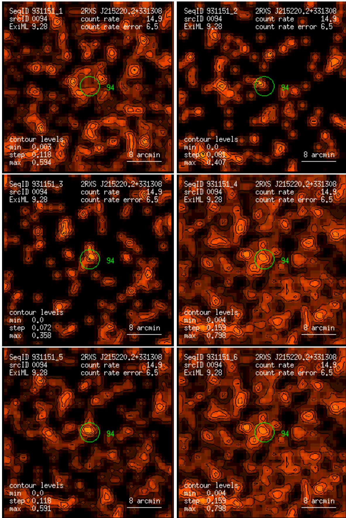
Figure 94: RASS 931151: detection 0094: band rate images, Gaussian filter: (1) PSPC channels 11 – 41, (2) 52 – 90, (3) 91 – 201, (4) 11 – 235, (5) 52 – 201, (6) 11 – 201. Broad band rates in counts/ks. Band rate contour levels in counts/ks/arcmin 2 .
