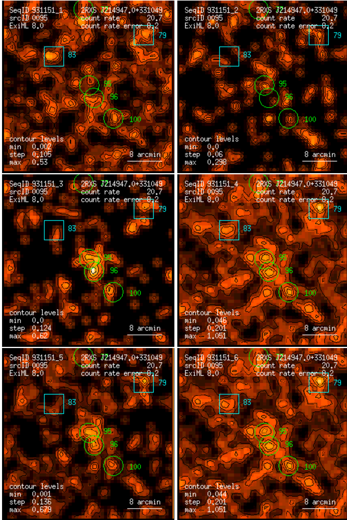
Figure 95: RASS 931151: detection 0095: band rate images, Gaussian filter: (1) PSPC channels 11 – 41, (2) 52 – 90, (3) 91 – 201, (4) 11 – 235, (5) 52 – 201, (6) 11 – 201. Broad band rates in counts/ks. Band rate contour levels in counts/ks/arcmin 2 .
