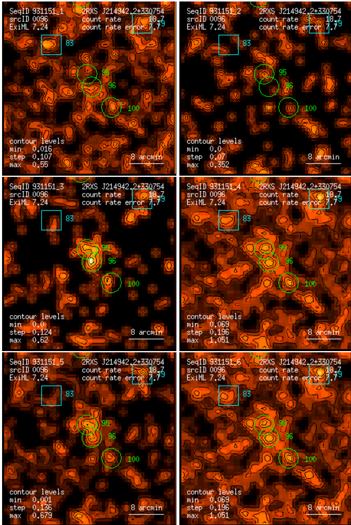
Figure 96: RASS 931151: detection 0096: band rate images, Gaussian filter: (1) PSPC channels 11 – 41, (2) 52 – 90, (3) 91 – 201, (4) 11 – 235, (5) 52 – 201, (6) 11 – 201. Broad band rates in counts/ks. Band rate contour levels in counts/ks/arcmin 2 .
