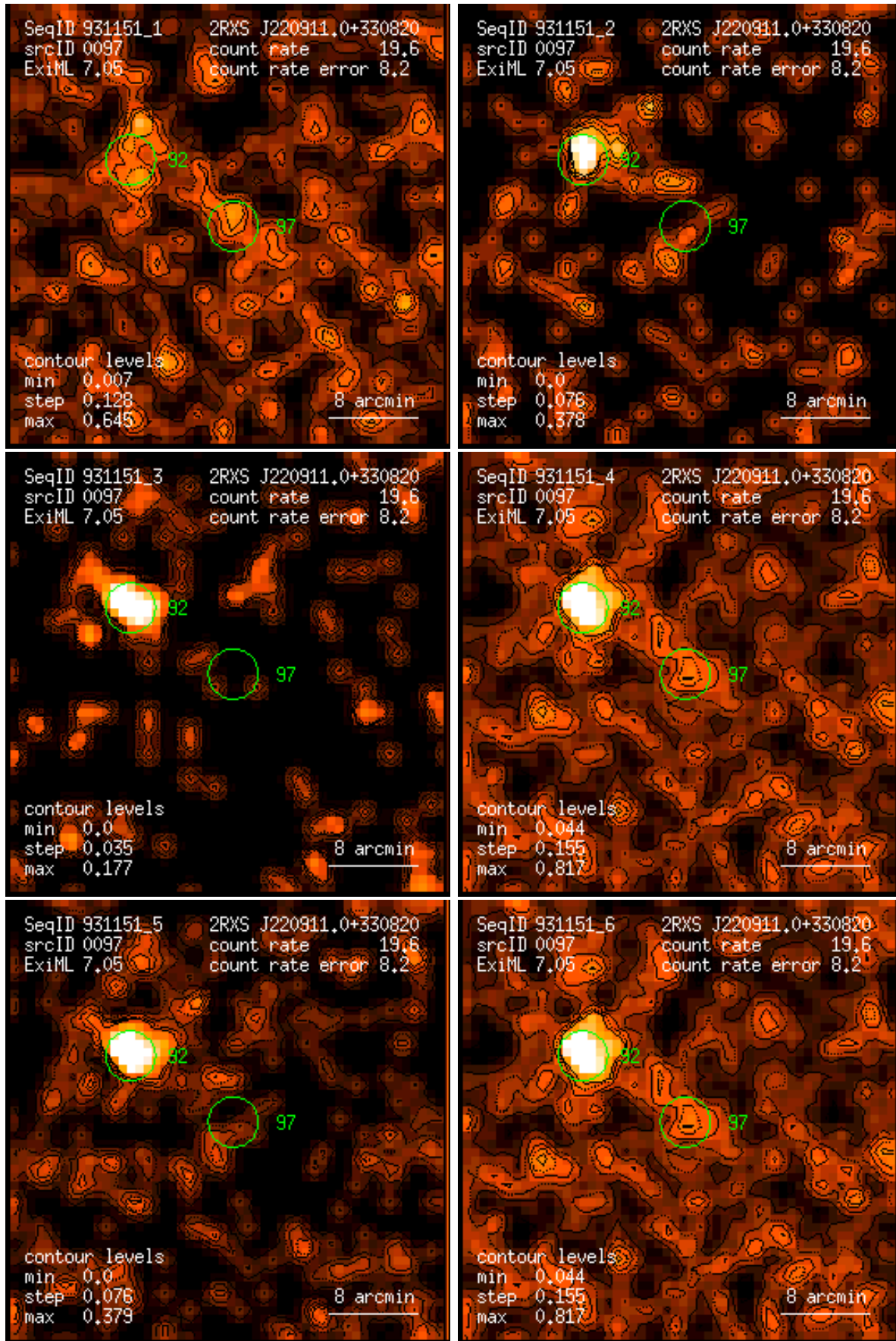
Figure 97: RASS 931151: detection 0097: band rate images, Gaussian filter: (1) PSPC channels 11 – 41, (2) 52 – 90, (3) 91 – 201, (4) 11 – 235, (5) 52 – 201, (6) 11 – 201. Broad band rates in counts/ks. Band rate contour levels in counts/ks/arcmin 2 .
