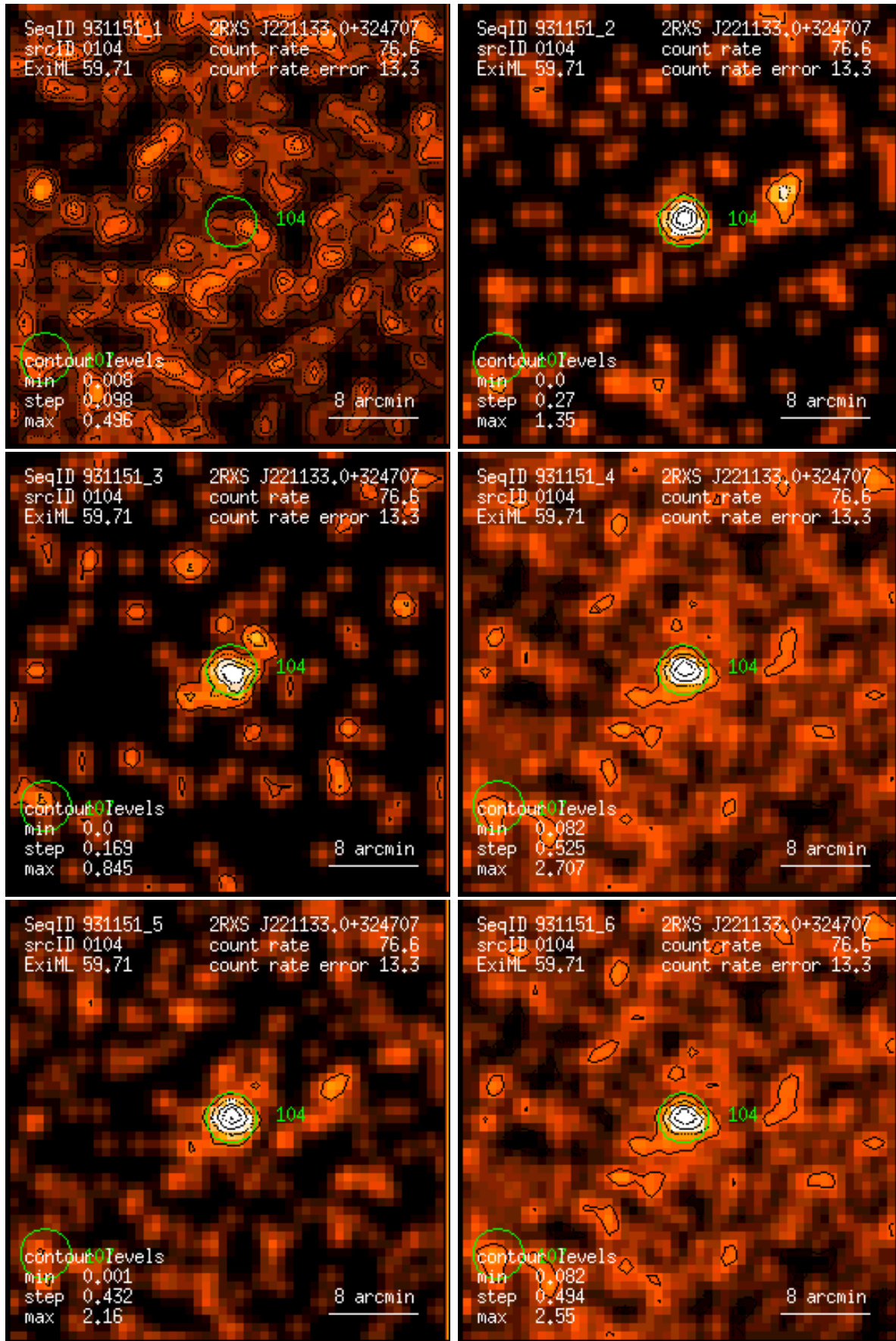
Figure 104: RASS 931151: detection 0104: band rate images, Gaussian filter: (1) PSPC channels 11 – 41, (2) 52 – 90, (3) 91 – 201, (4) 11 – 235, (5) 52 – 201, (6) 11 – 201. Broad band rates in counts/ks. Band rate contour levels in counts/ks/arcmin 2 .
