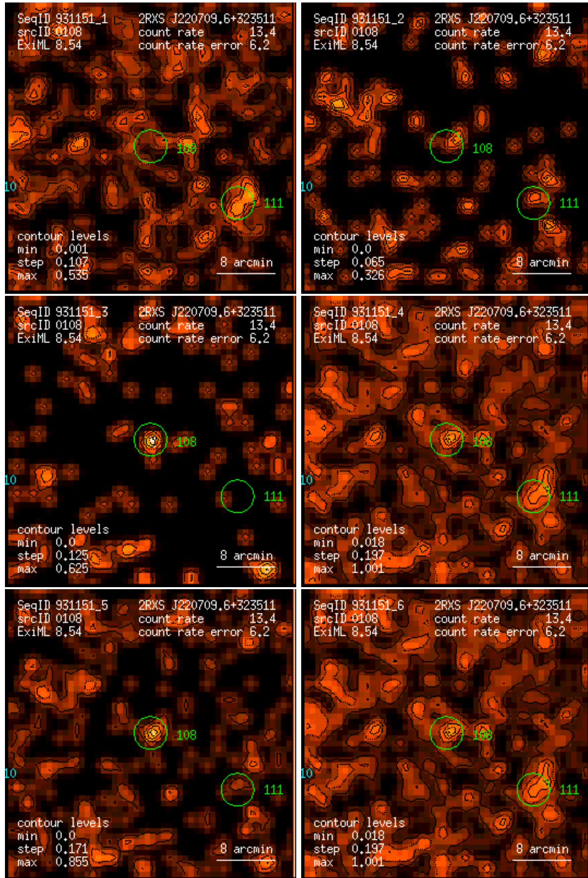
Figure 108: RASS 931151: detection 0108: band rate images, Gaussian filter: (1) PSPC channels 11 – 41, (2) 52 – 90, (3) 91 – 201, (4) 11 – 235, (5) 52 – 201, (6) 11 – 201. Broad band rates in counts/ks. Band rate contour levels in counts/ks/arcmin 2 .
