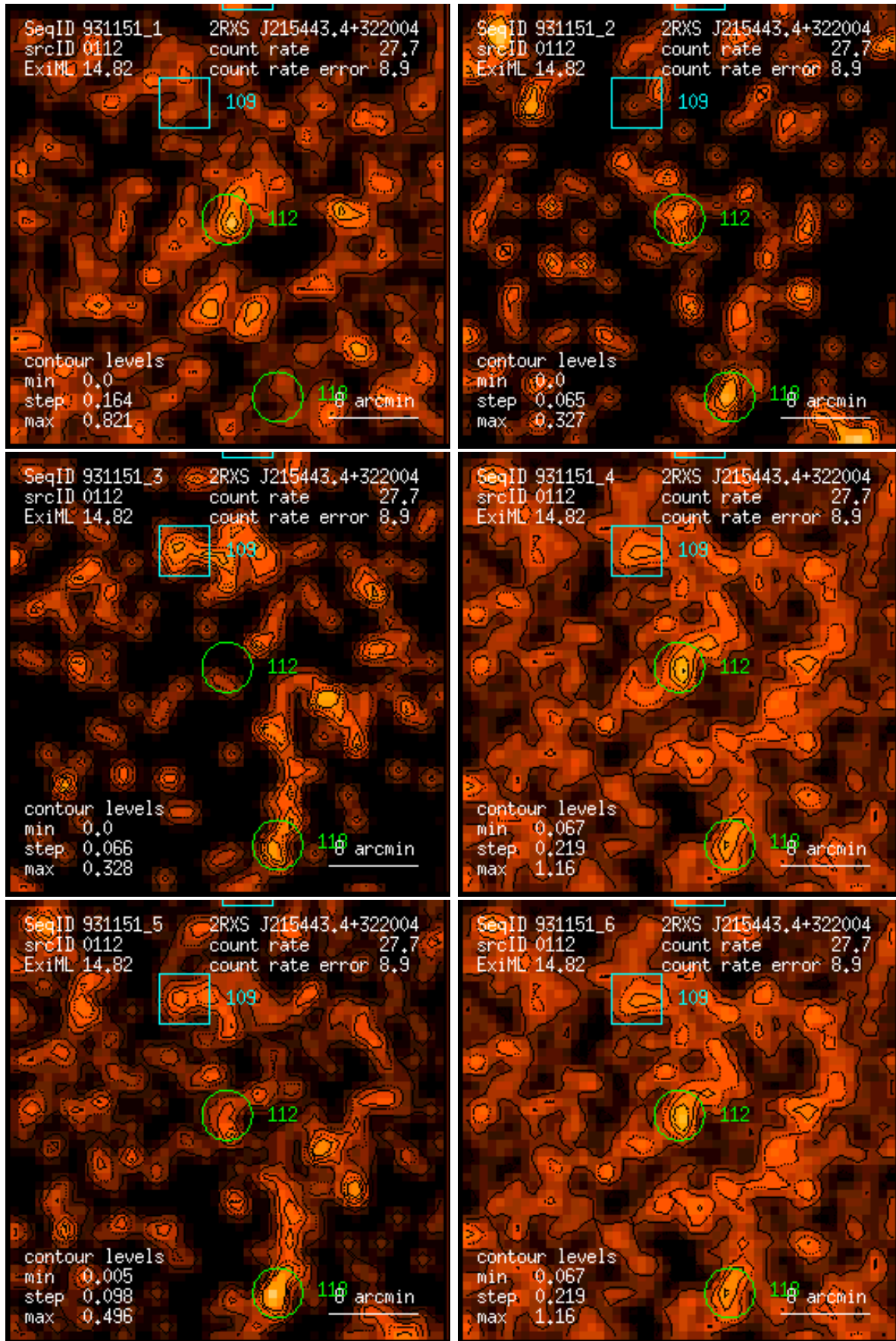
Figure 112: RASS 931151: detection 0112: band rate images, Gaussian filter: (1) PSPC channels 11 – 41, (2) 52 – 90, (3) 91 – 201, (4) 11 – 235, (5) 52 – 201, (6) 11 – 201. Broad band rates in counts/ks. Band rate contour levels in counts/ks/arcmin 2 .
