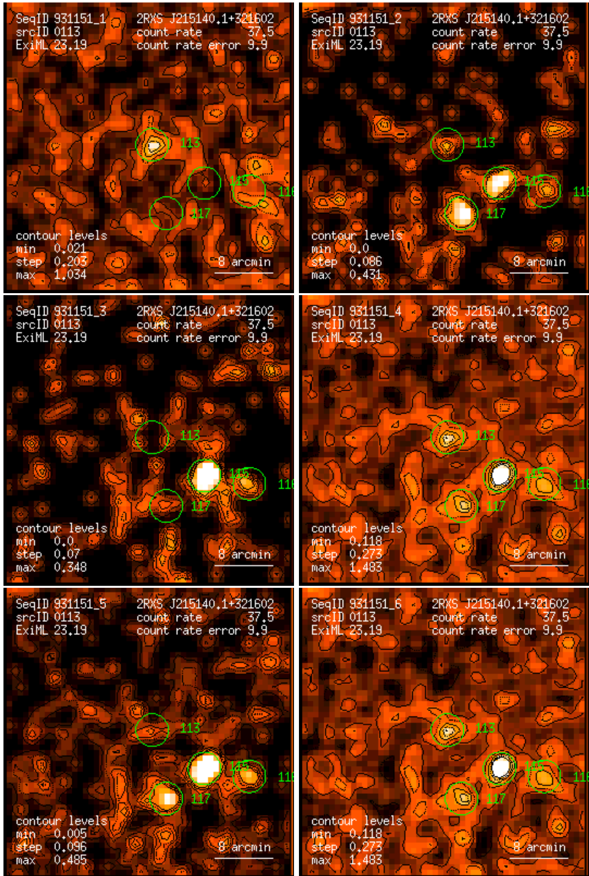
Figure 113: RASS 931151: detection 0113: band rate images, Gaussian filter: (1) PSPC channels 11 – 41, (2) 52 – 90, (3) 91 – 201, (4) 11 – 235, (5) 52 – 201, (6) 11 – 201. Broad band rates in counts/ks. Band rate contour levels in counts/ks/arcmin 2 .
