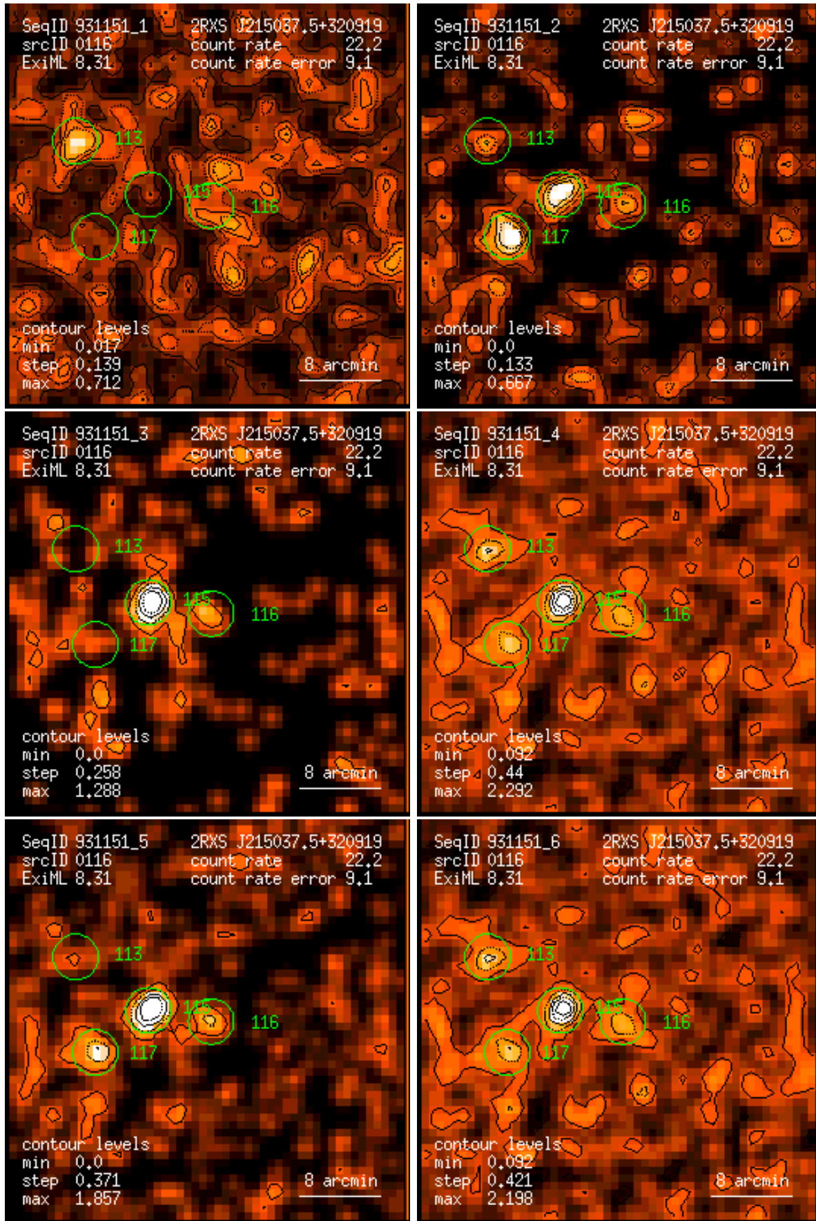
Figure 116: RASS 931151: detection 0116: band rate images, Gaussian filter: (1) PSPC channels 11 – 41, (2) 52 – 90, (3) 91 – 201, (4) 11 – 235, (5) 52 – 201, (6) 11 – 201. Broad band rates in counts/ks. Band rate contour levels in counts/ks/arcmin 2 .
