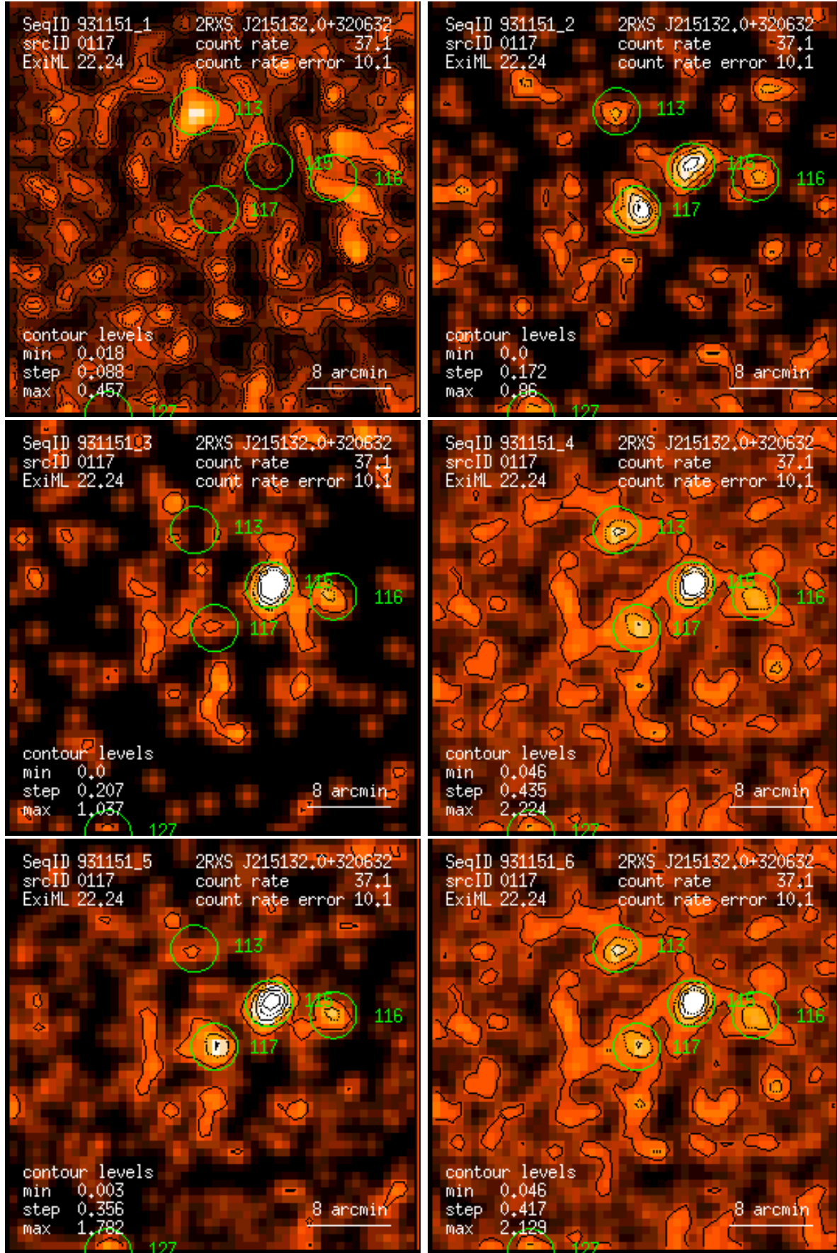
Figure 117: RASS 931151: detection 0117: band rate images, Gaussian filter: (1) PSPC channels 11 – 41, (2) 52 – 90, (3) 91 – 201, (4) 11 – 235, (5) 52 – 201, (6) 11 – 201. Broad band rates in counts/ks. Band rate contour levels in counts/ks/arcmin 2 .
