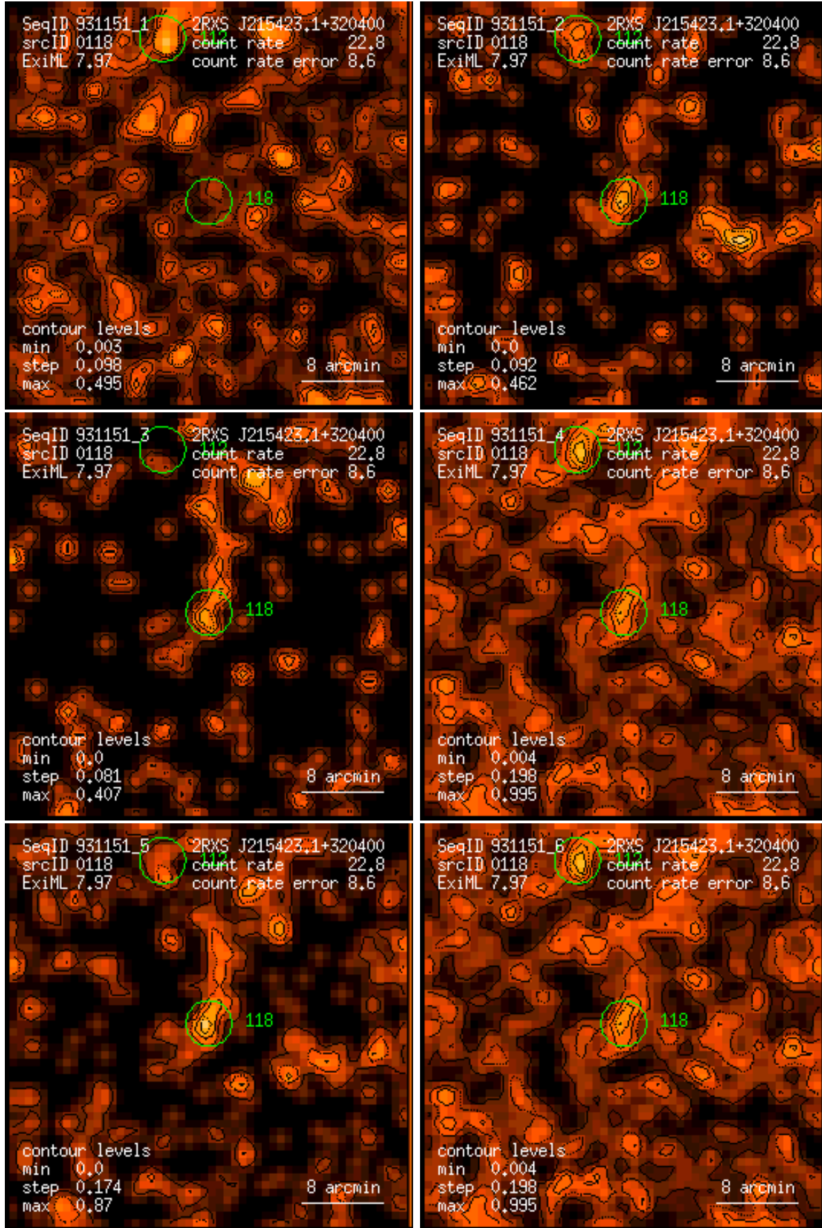
Figure 118: RASS 931151: detection 0118: band rate images, Gaussian filter: (1) PSPC channels 11 – 41, (2) 52 – 90, (3) 91 – 201, (4) 11 – 235, (5) 52 – 201, (6) 11 – 201. Broad band rates in counts/ks. Band rate contour levels in counts/ks/arcmin 2 .
