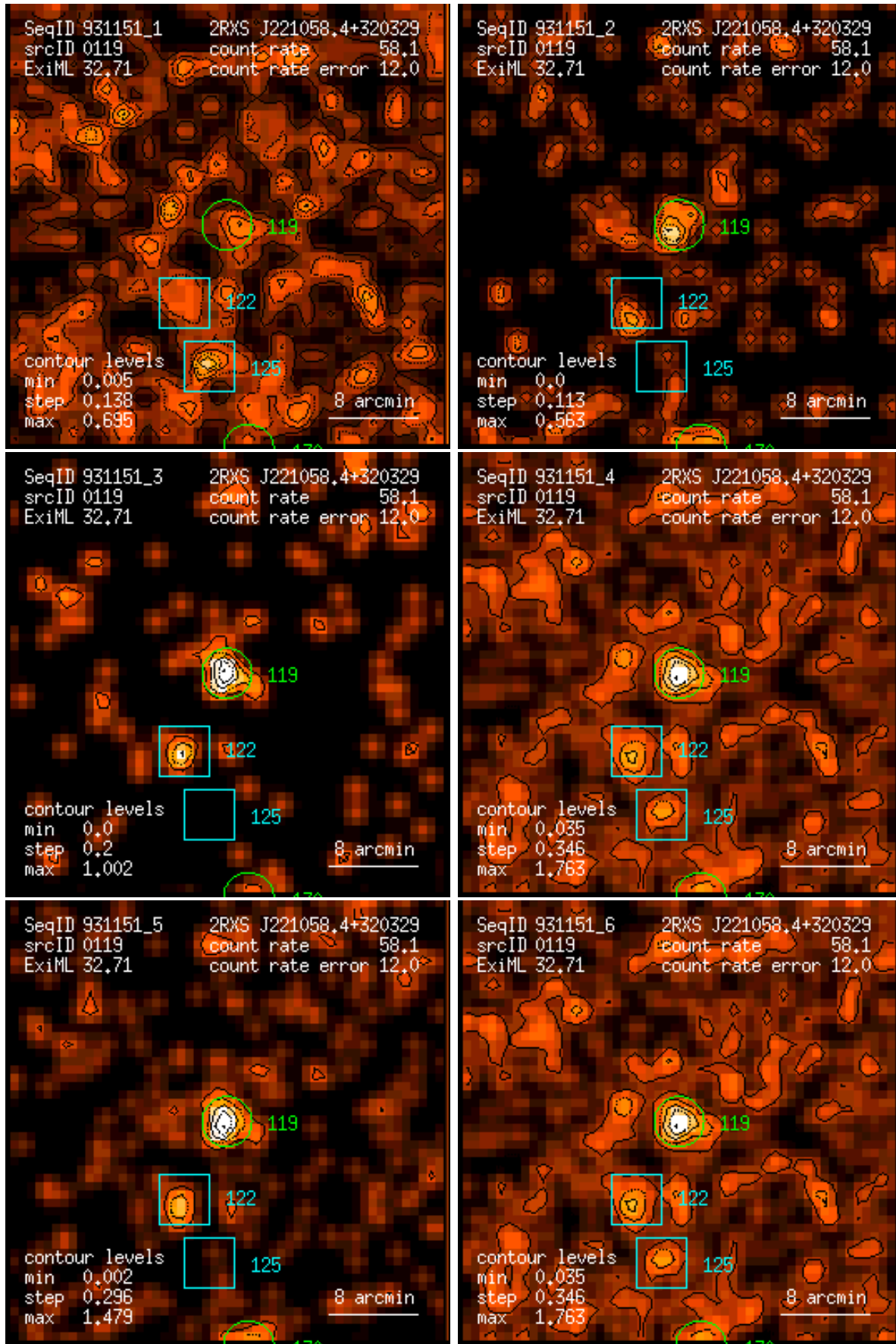
Figure 119: RASS 931151: detection 0119: band rate images, Gaussian filter: (1) PSPC channels 11 – 41, (2) 52 – 90, (3) 91 – 201, (4) 11 – 235, (5) 52 – 201, (6) 11 – 201. Broad band rates in counts/ks. Band rate contour levels in counts/ks/arcmin 2 .
