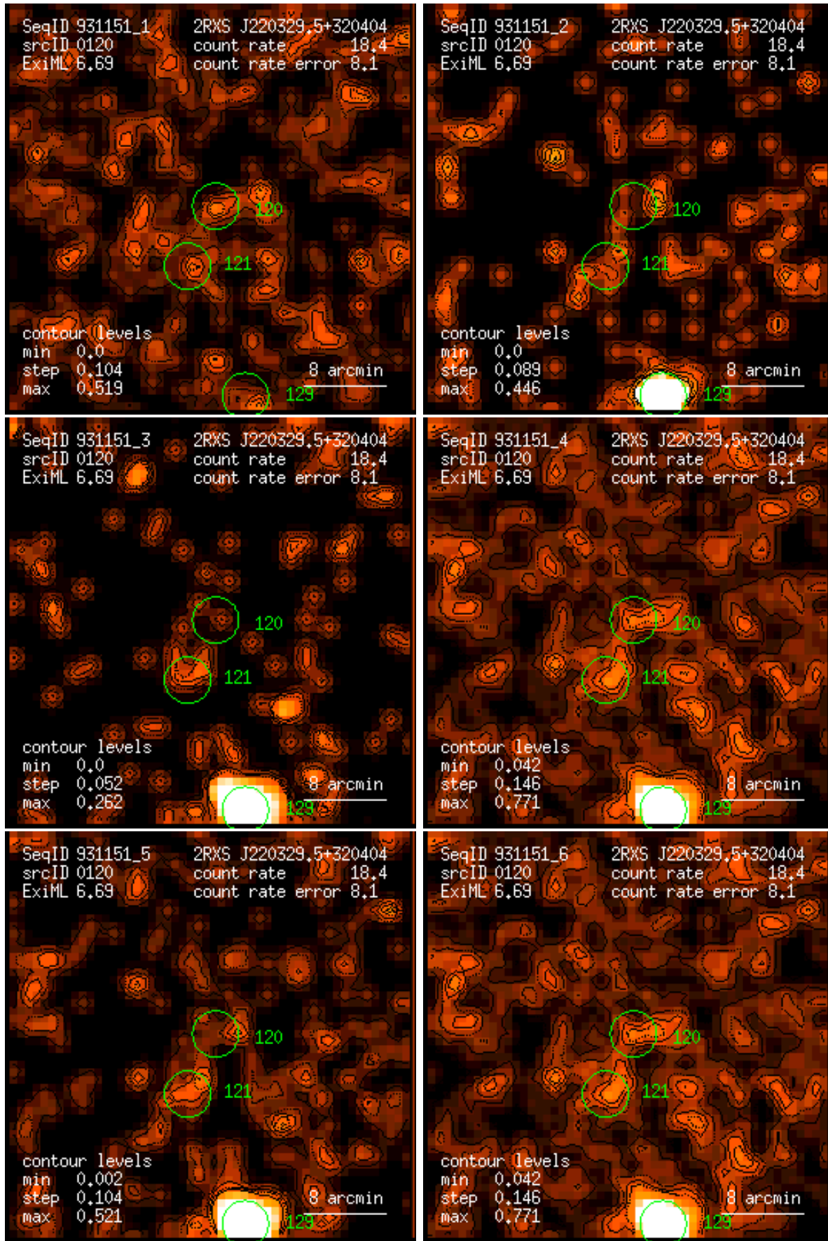
Figure 120: RASS 931151: detection 0120: band rate images, Gaussian filter: (1) PSPC channels 11 – 41, (2) 52 – 90, (3) 91 – 201, (4) 11 – 235, (5) 52 – 201, (6) 11 – 201. Broad band rates in counts/ks. Band rate contour levels in counts/ks/arcmin 2 .
