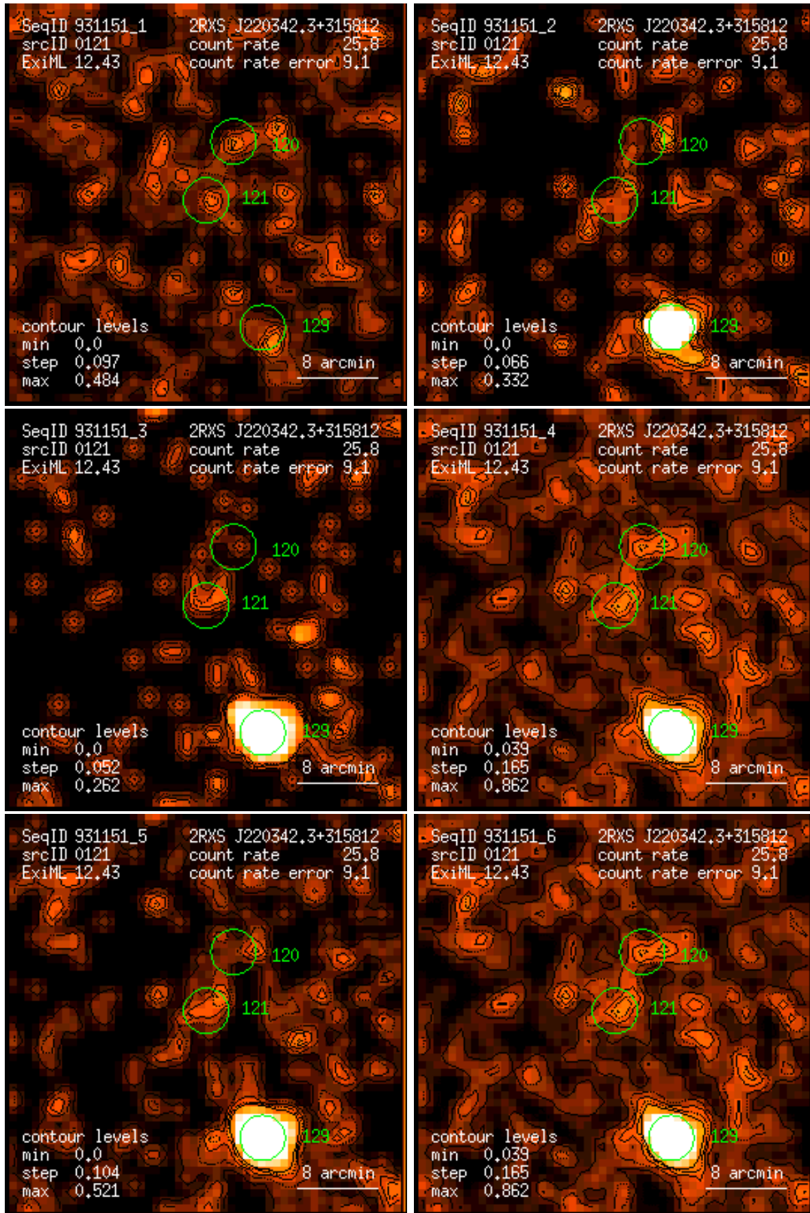
Figure 121: RASS 931151: detection 0121: band rate images, Gaussian filter: (1) PSPC channels 11 – 41, (2) 52 – 90, (3) 91 – 201, (4) 11 – 235, (5) 52 – 201, (6) 11 – 201. Broad band rates in counts/ks. Band rate contour levels in counts/ks/arcmin 2 .
